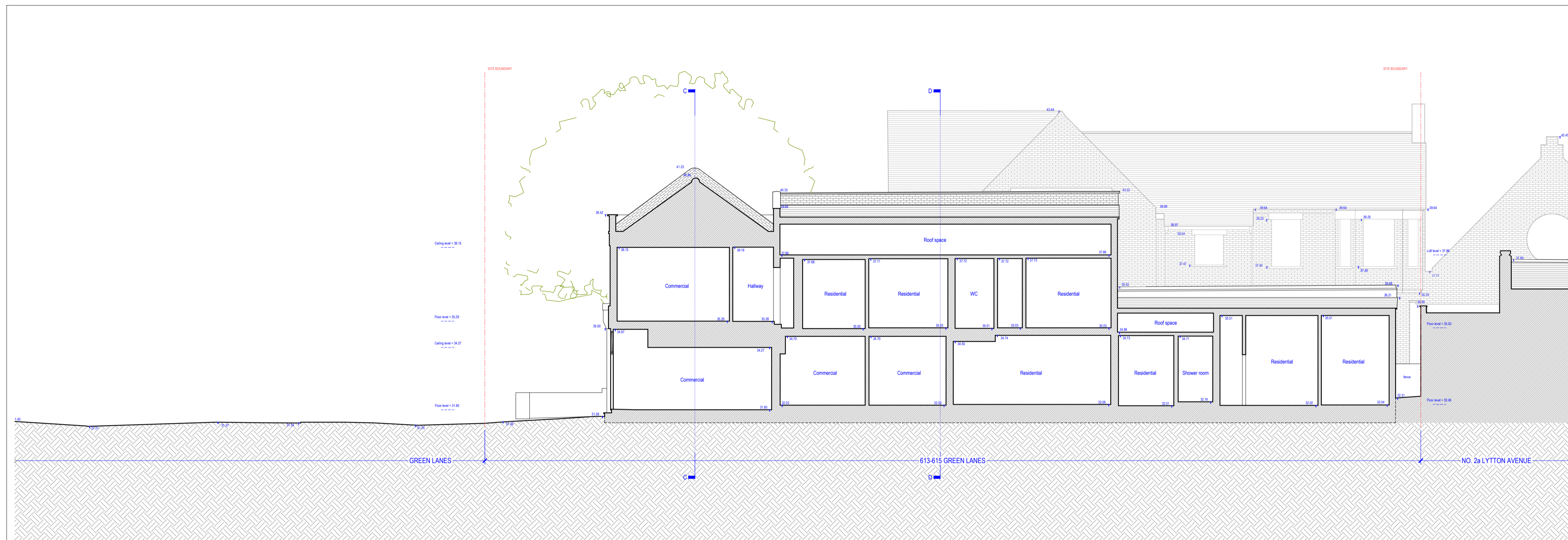
[01] EXISTING SECTION B-B
