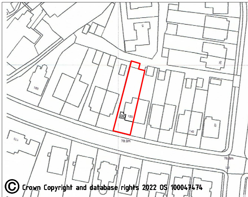
PROPOSED LOCATION PLAN 1:1250
