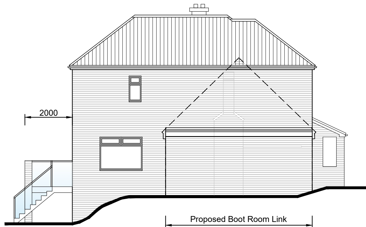
NORTH Elevation
