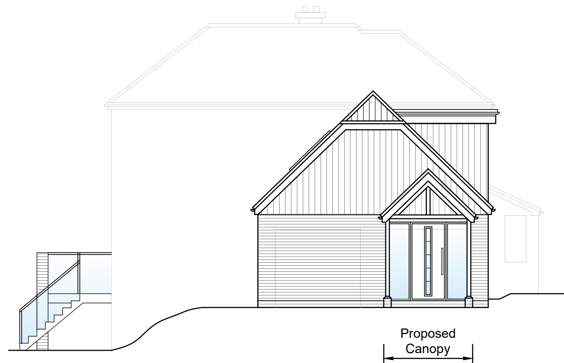
NORTH GARAGE Elevation
