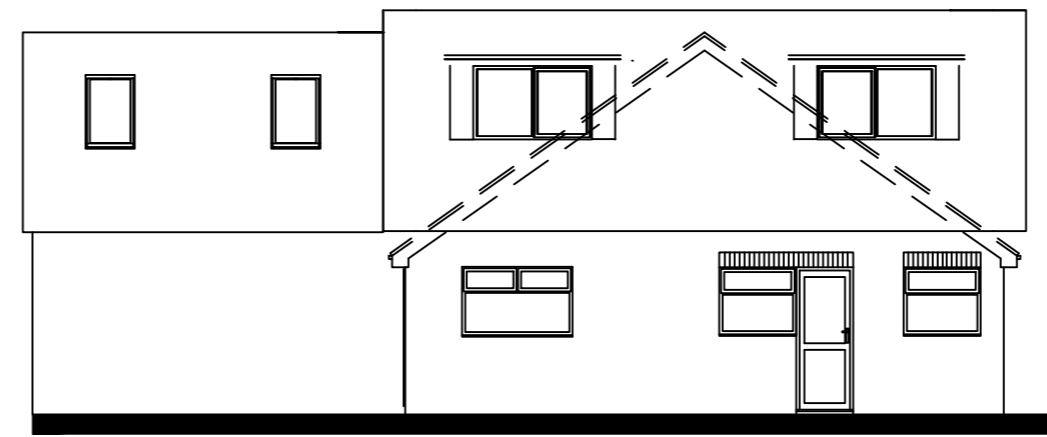
Western elevation
