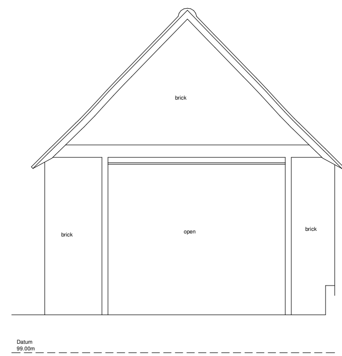
WEST ELEVATION
