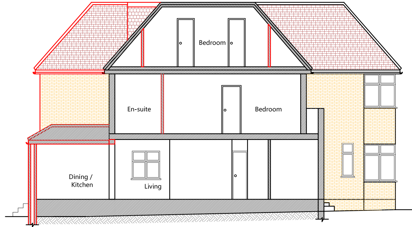
Proposed Section x-x
