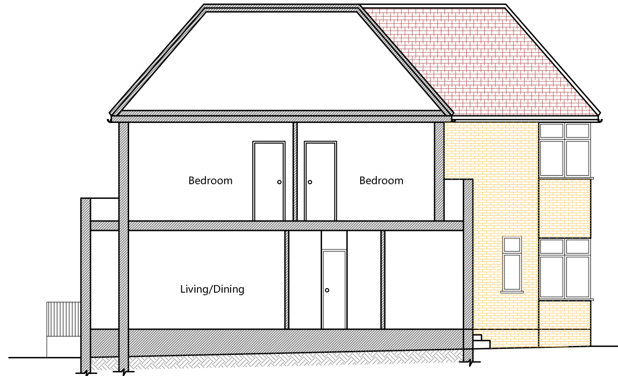
Existing Section x-x
