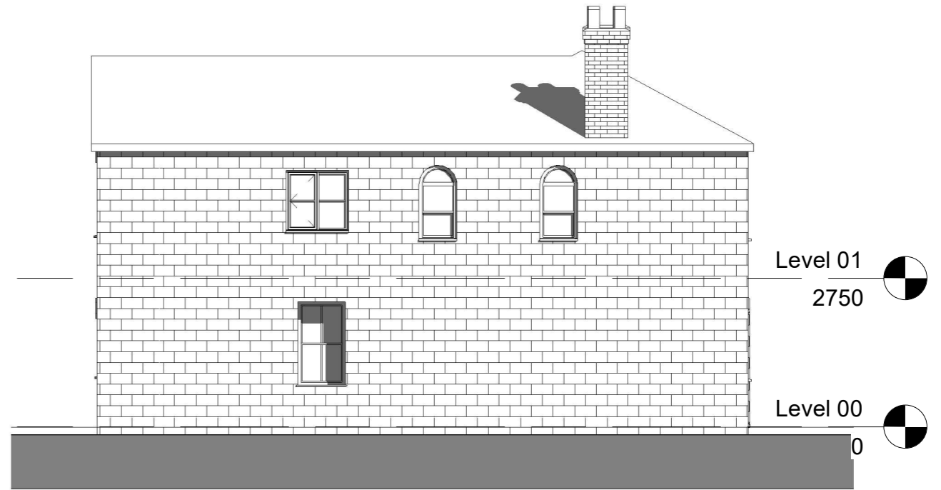
West Elevation 1 : 100
