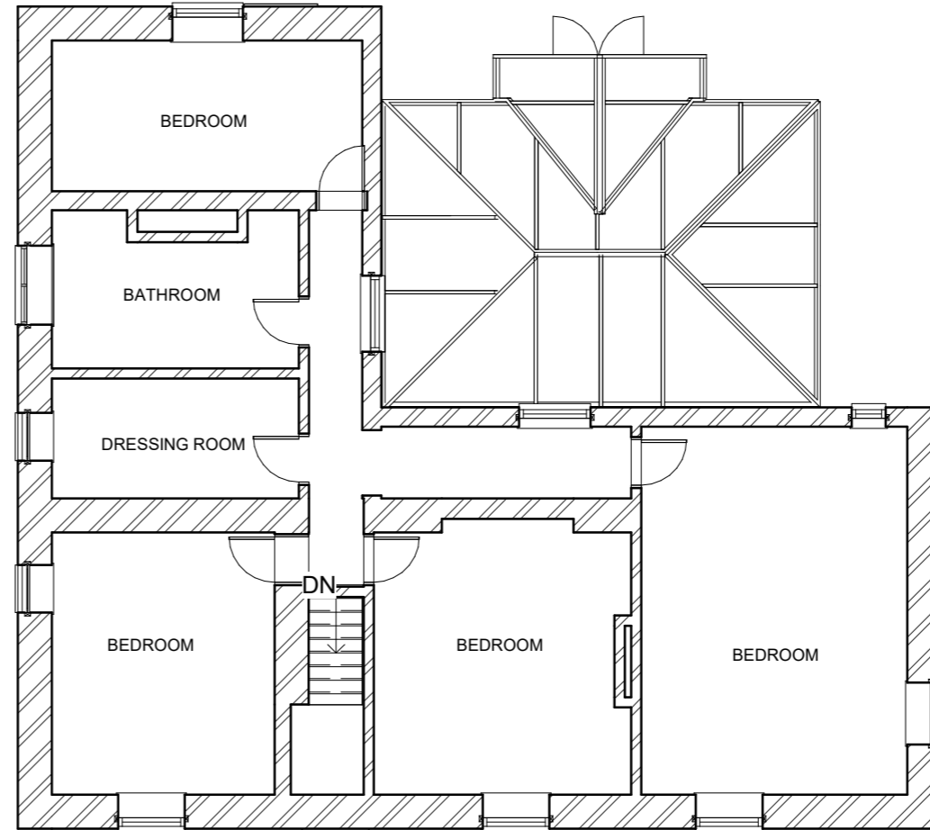
Level 01
