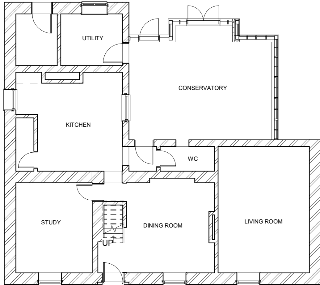
Level 00
