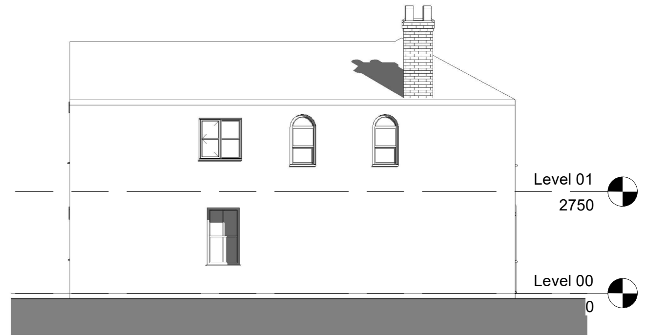
West Elevation 1 : 100
