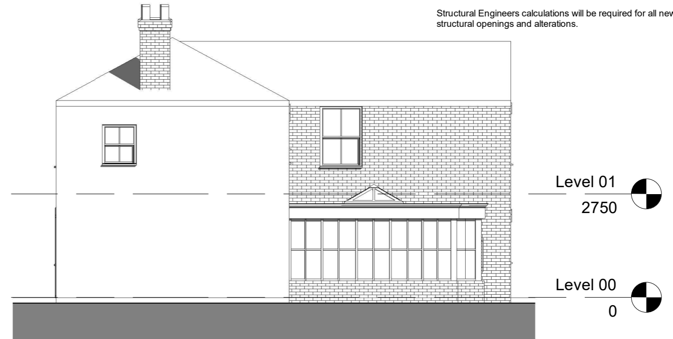
East Elevation 1 : 100
