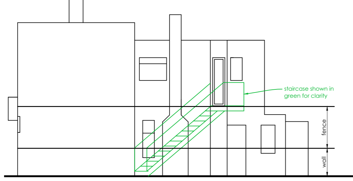
Proposed flank elevation
