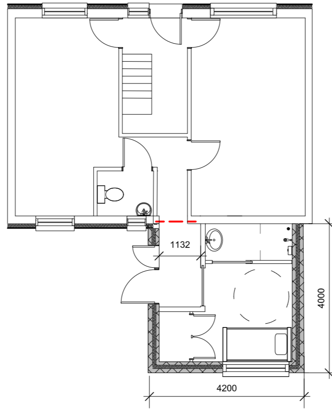
Proposed Floor Plan
