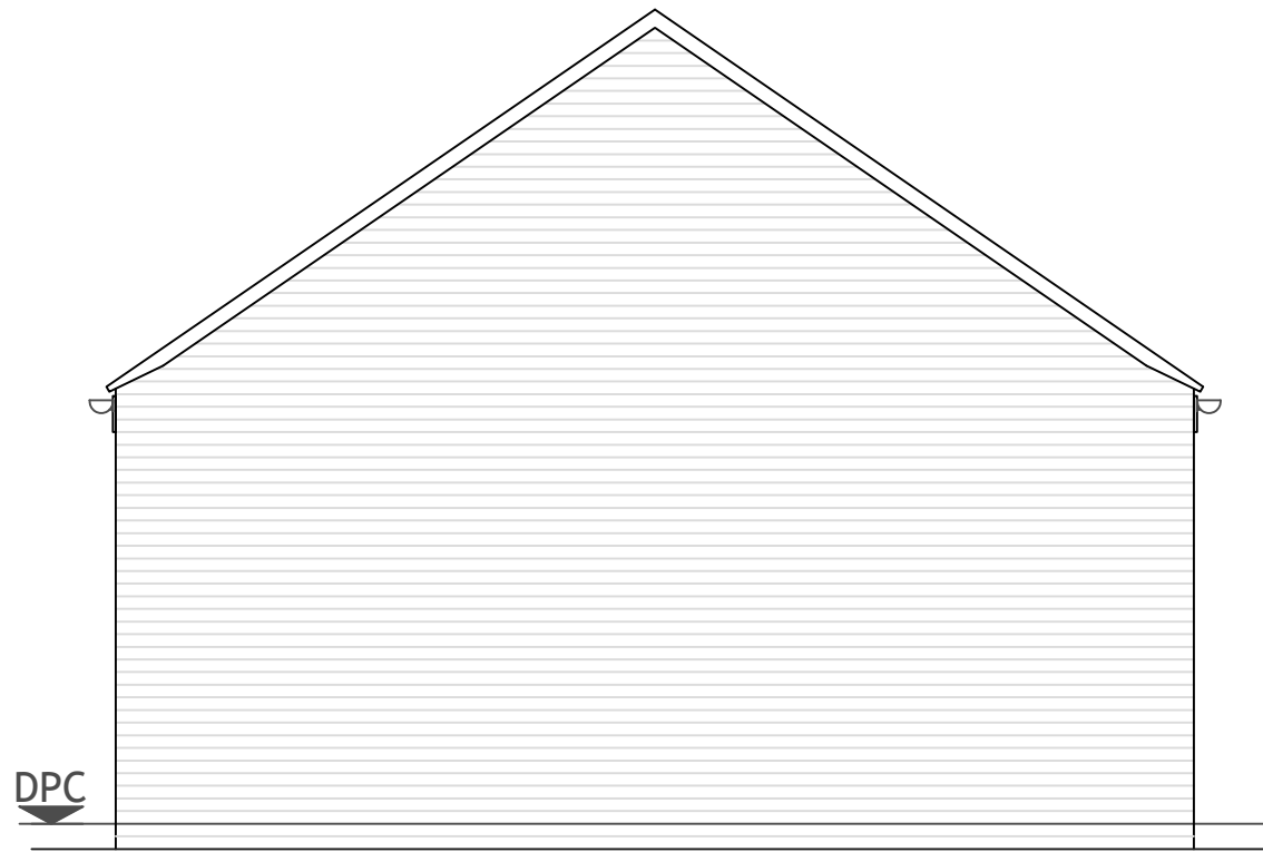
Single Garage Side Elevation 1:50
