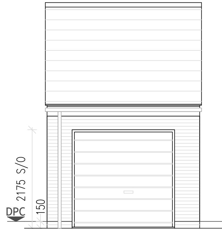
Single Garage Front Elevation 1:50
