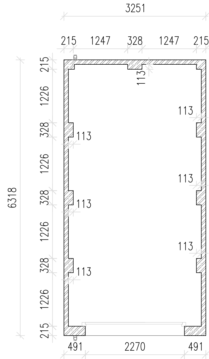
Single Garage Plan 1:50
