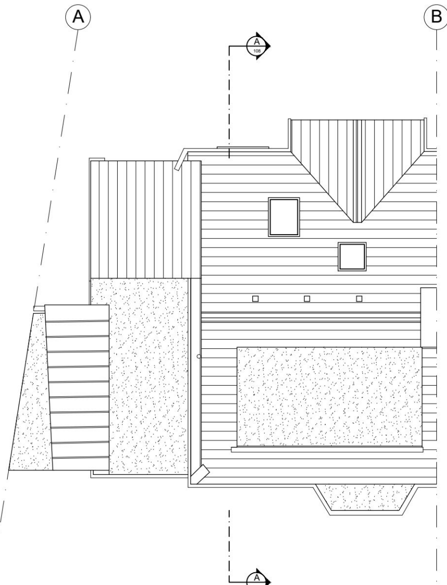
Roof Plan
