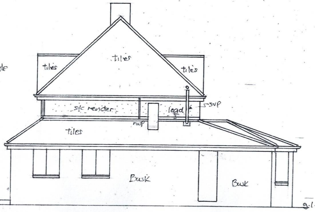
Gable Elevation Existing
