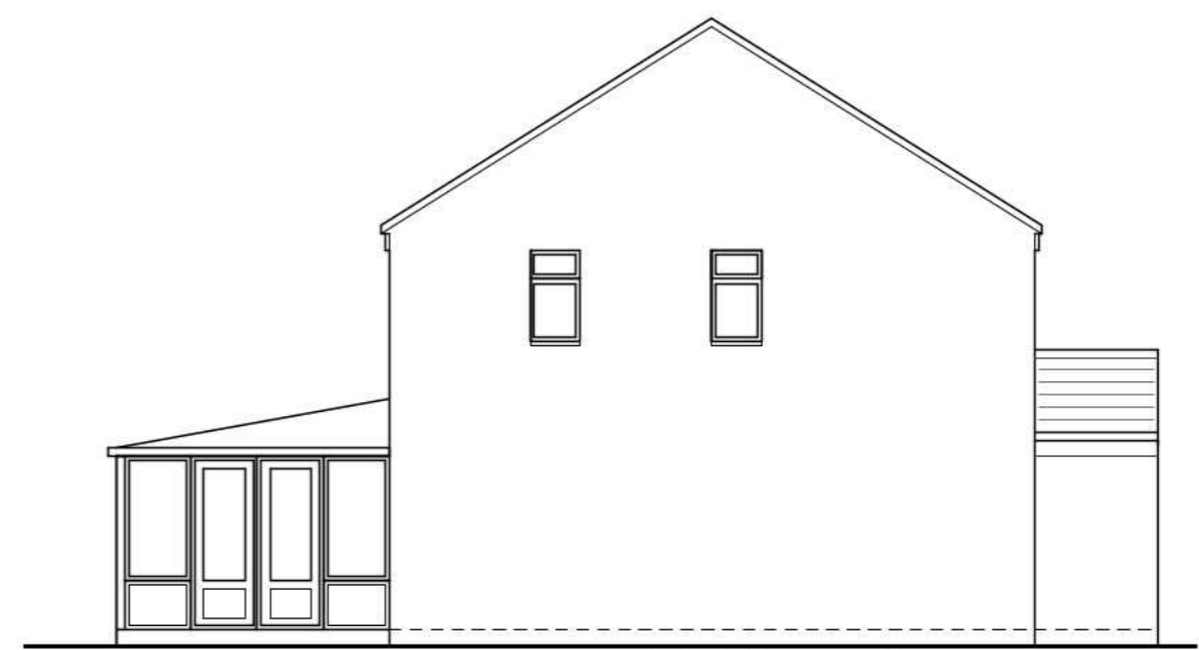
left side (southeast) elevation
