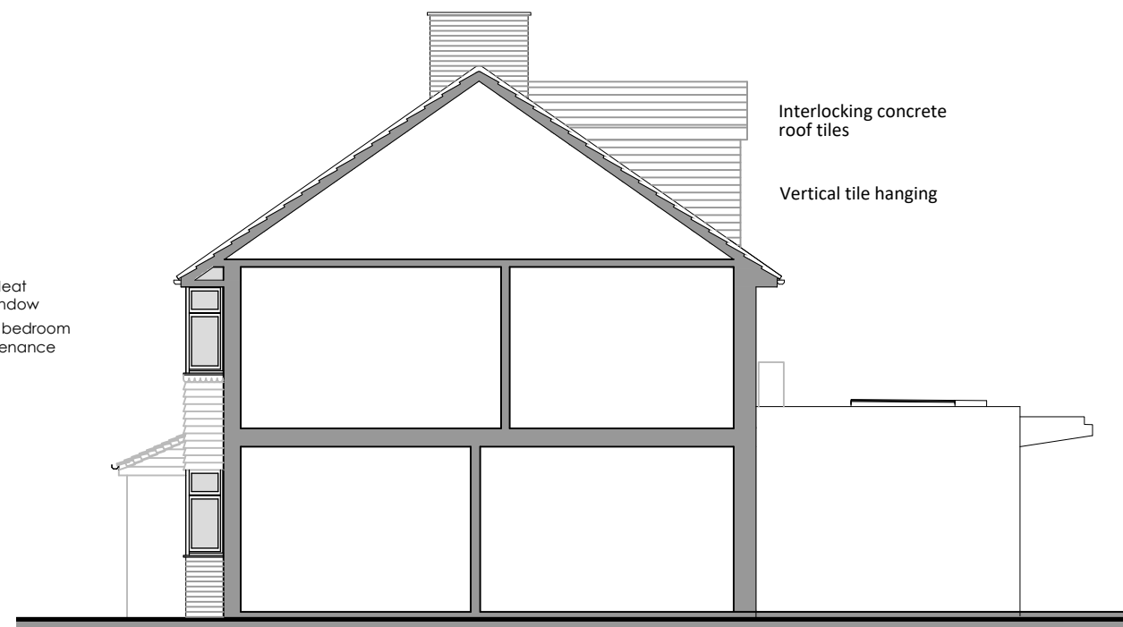
North West Sectional Elevation
