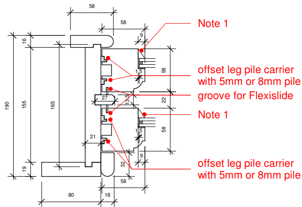
Plan Detail 1:5
