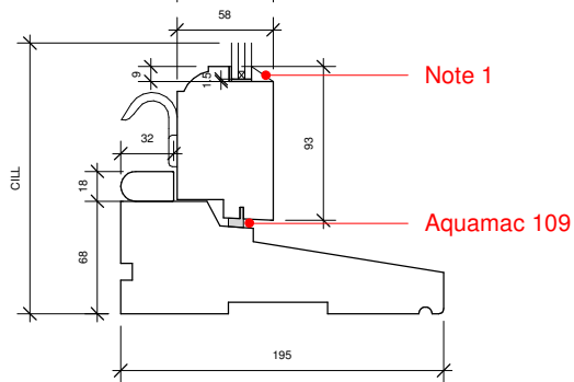
Sectional Detail 1:5
