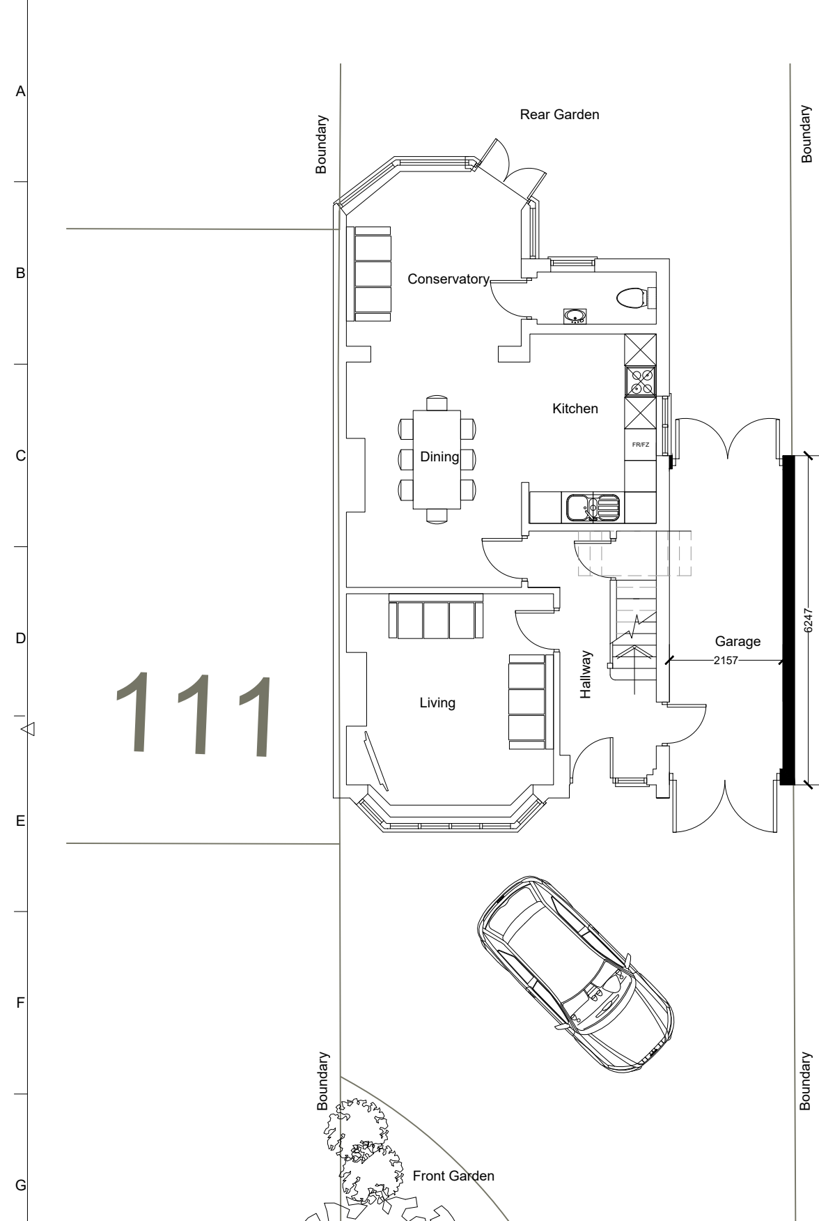
1 GROUND FLOOR PLAN - PROPOSED Scale: 1:100
