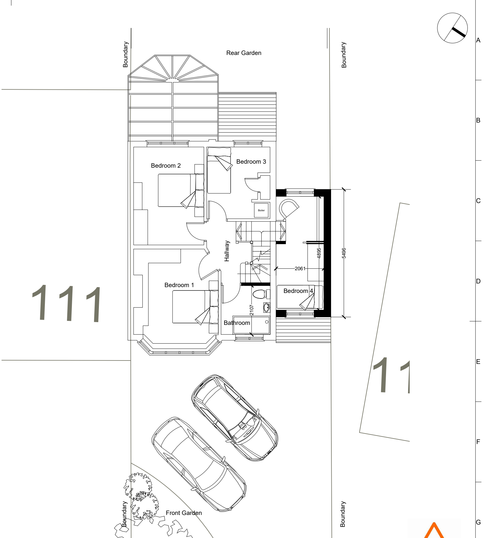
2 FIRST FLOOR PLAN - PROPOSED Scale: 1:100
