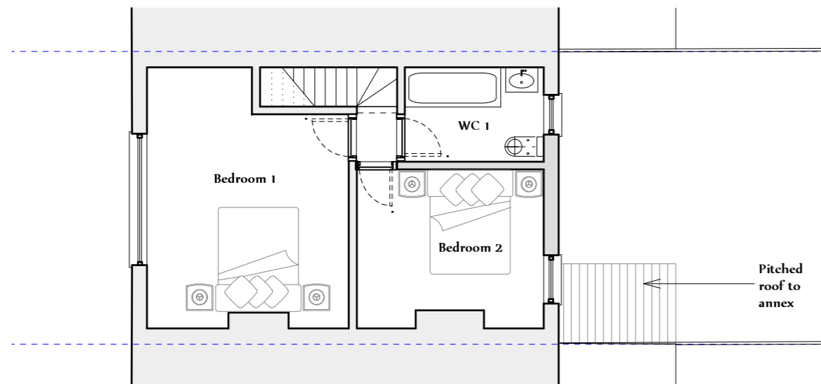
EXISTING FIRST FLOOR PLAN SCALE 1:100 @ A3
