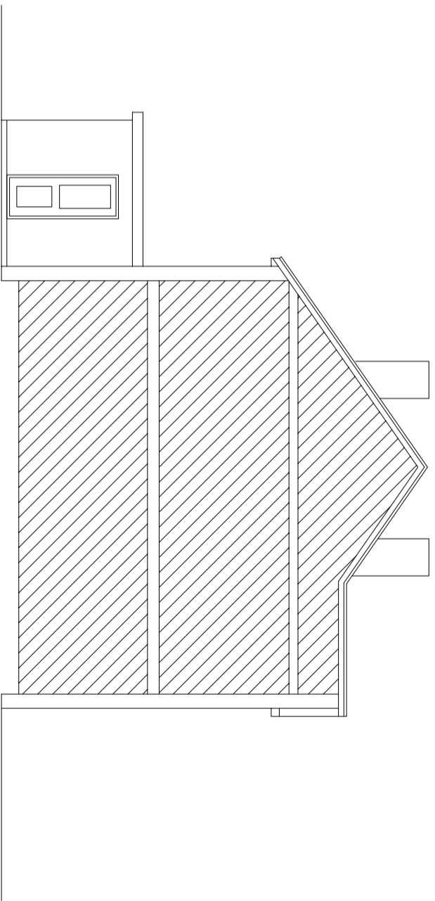
EXISTING SIDE SECTIONAL ELEVATION
