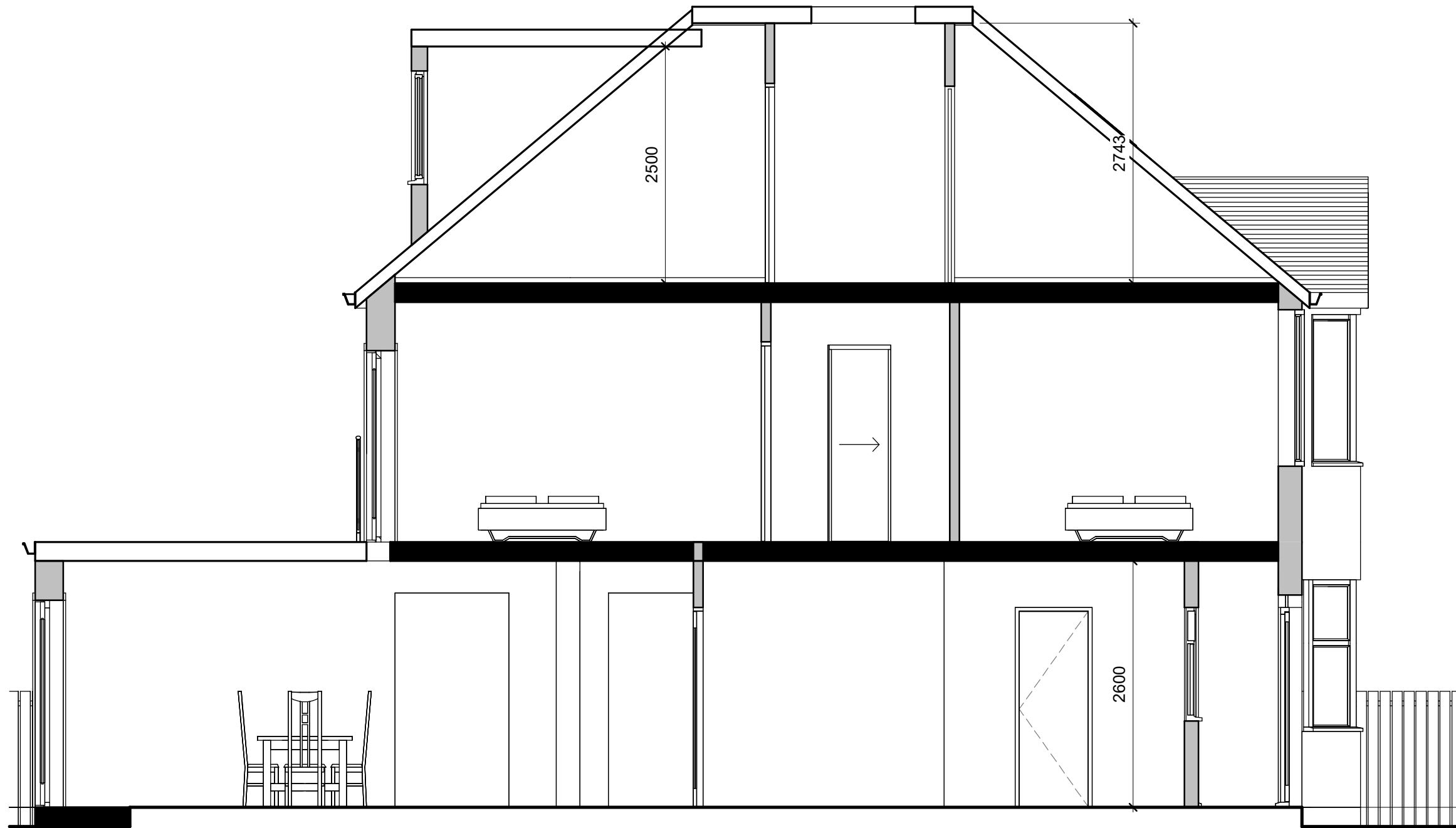
Proposed Section A-A 1 : 50
