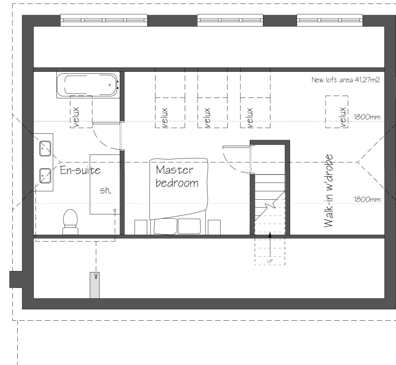
Second Floor & Roof Plan
