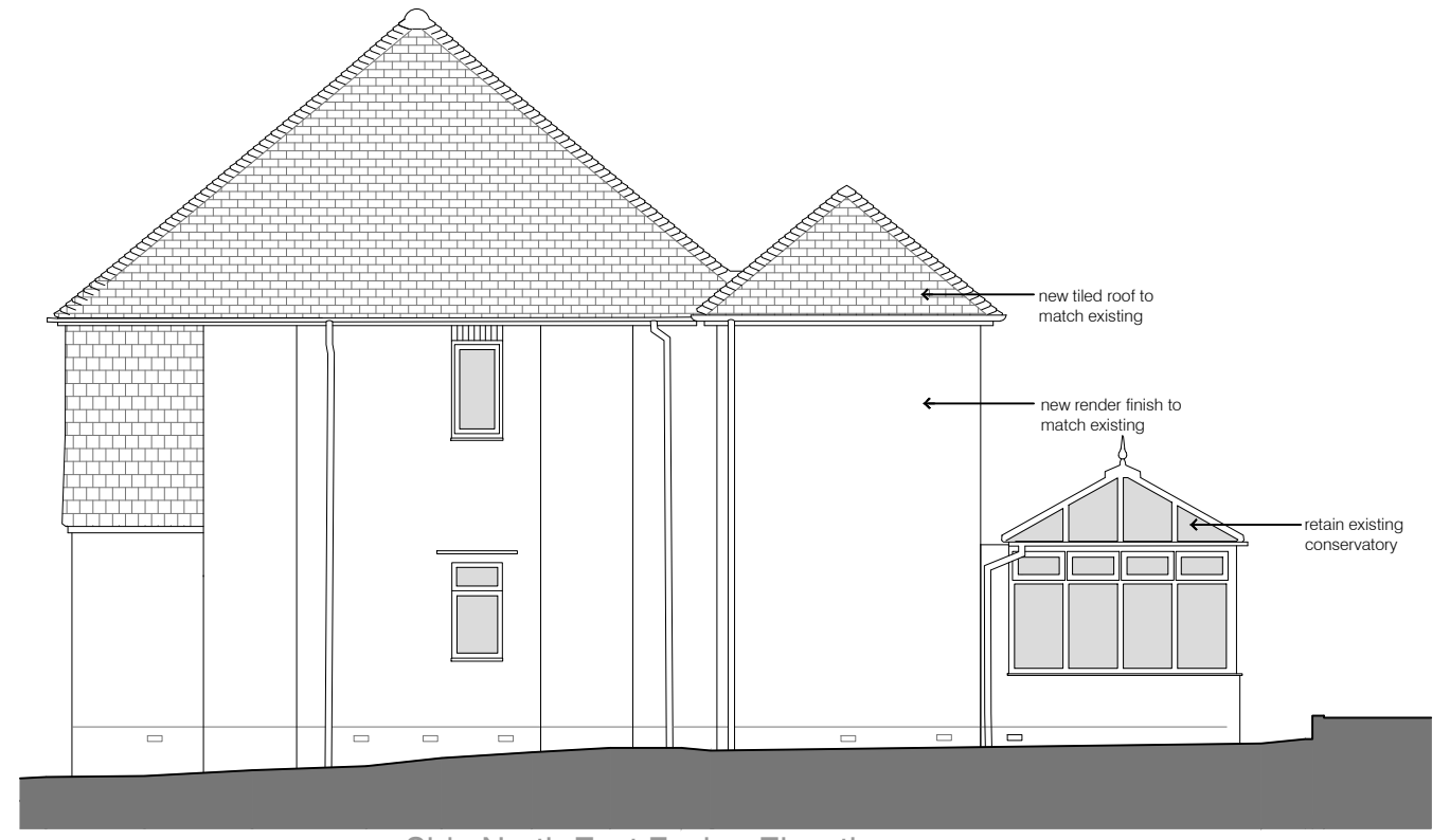
Side North East Facing Elevation
