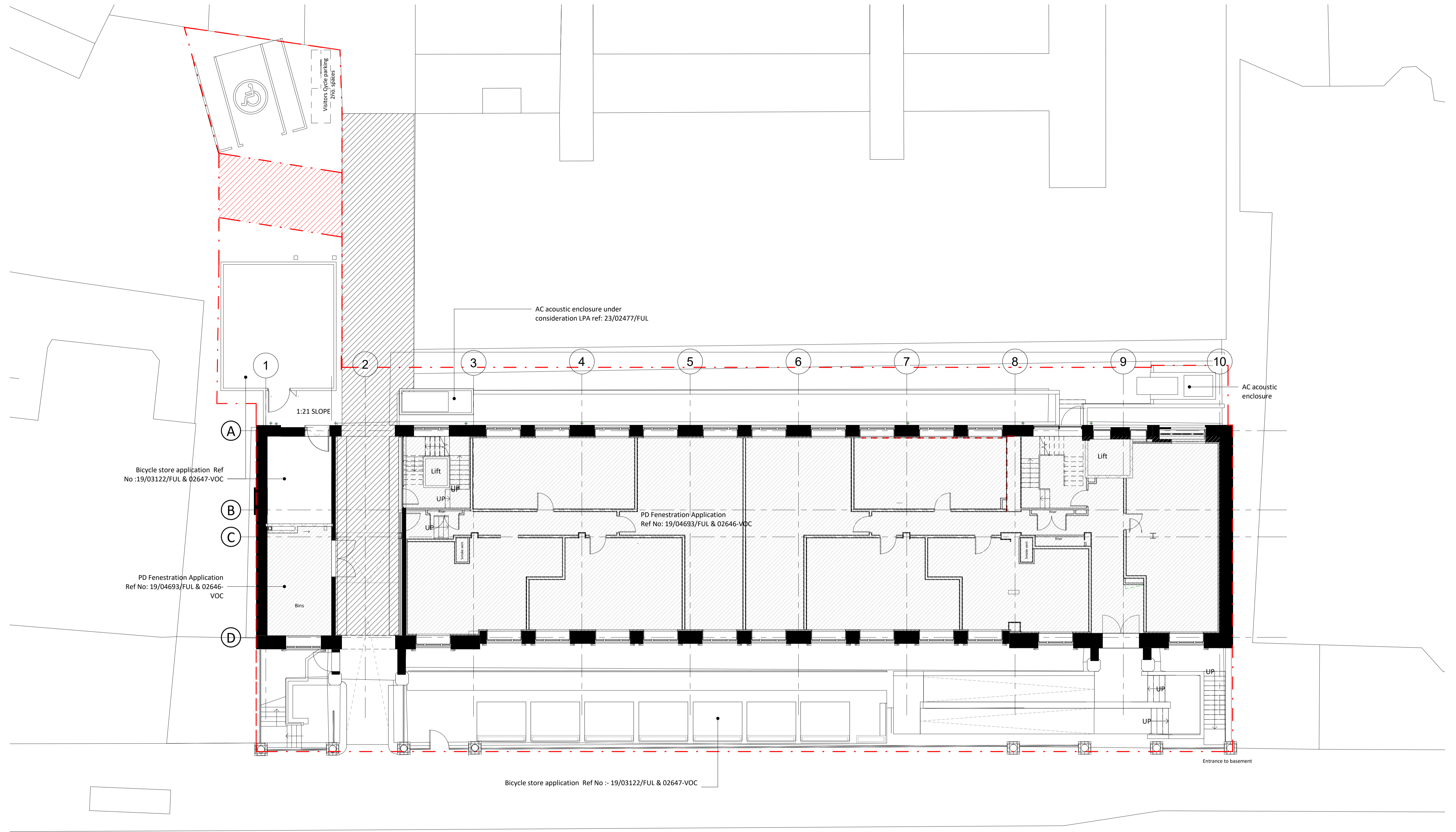
1 L00-Ground Floor Core A 1 : 100
