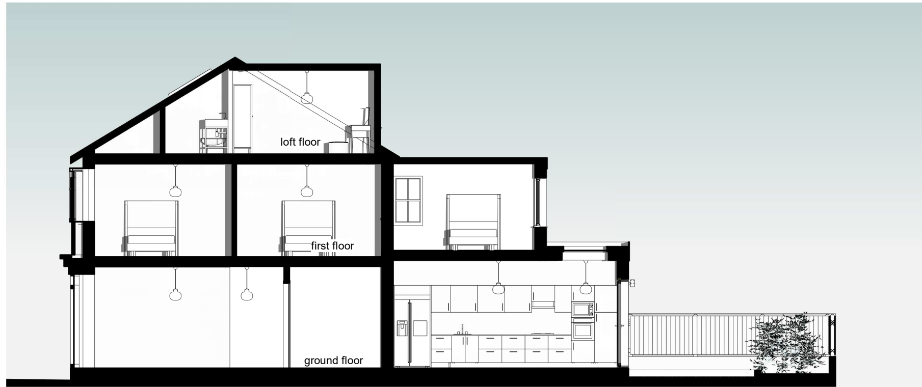
1 | PROPOSED B-B SECTION 1 : 100
