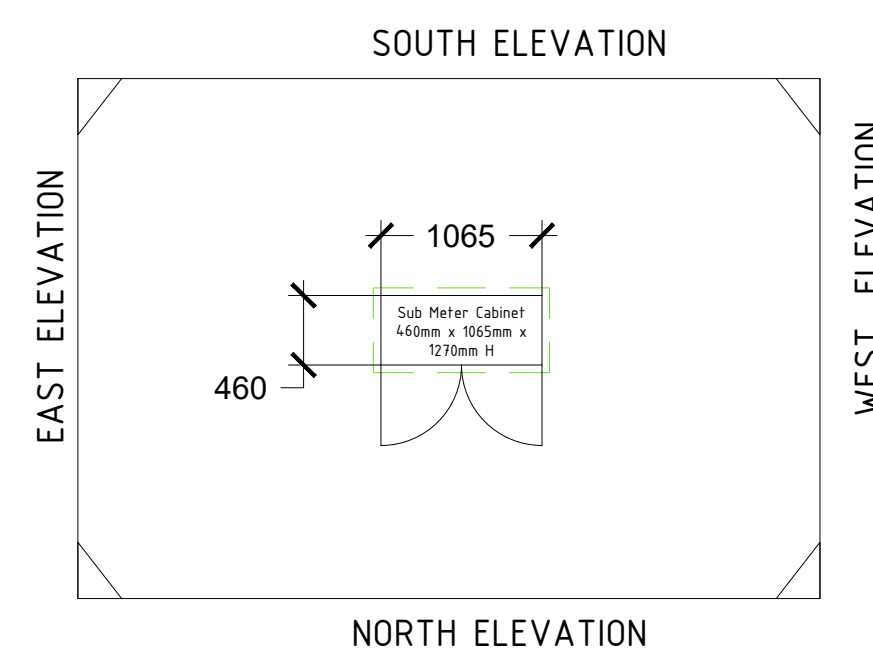
South Elevation North Elevation East & West Elevation Scale 1:50 Scale 1:50 Scale 1:50
