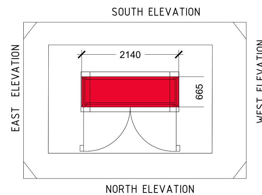
Low Voltage (LV) Feeder Pillar Floor Plan Scale 1:50
