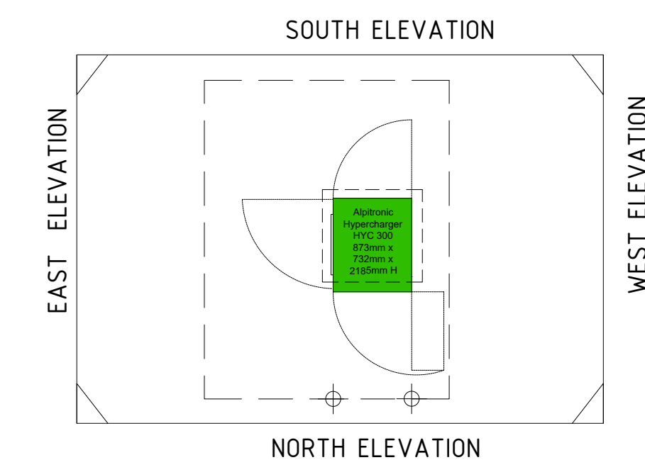
Alpitronic Hypercharger HYC 300 POWER CABINET & CHARGER Floor Plan Scale 1:50
