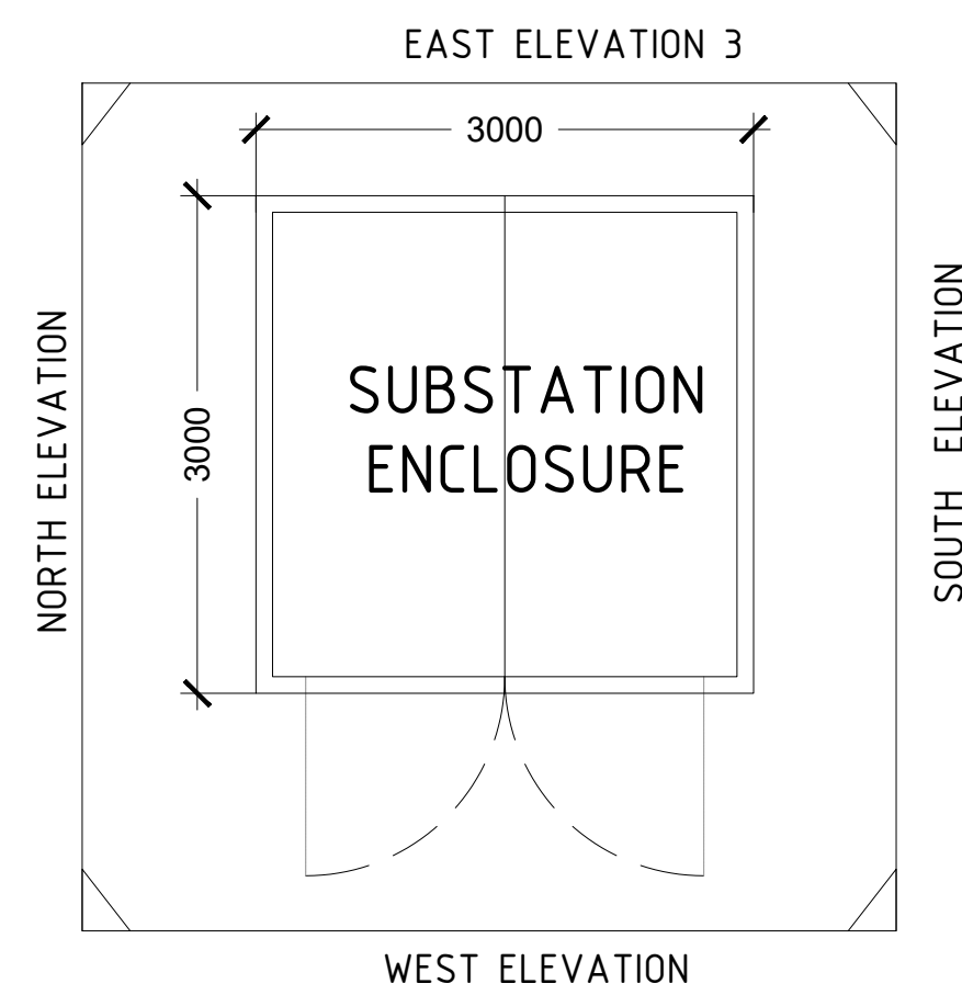
GRP Substation Floor Plan Scale 1:50
