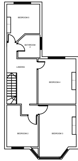
PROPOSED FIRST FLOOR
