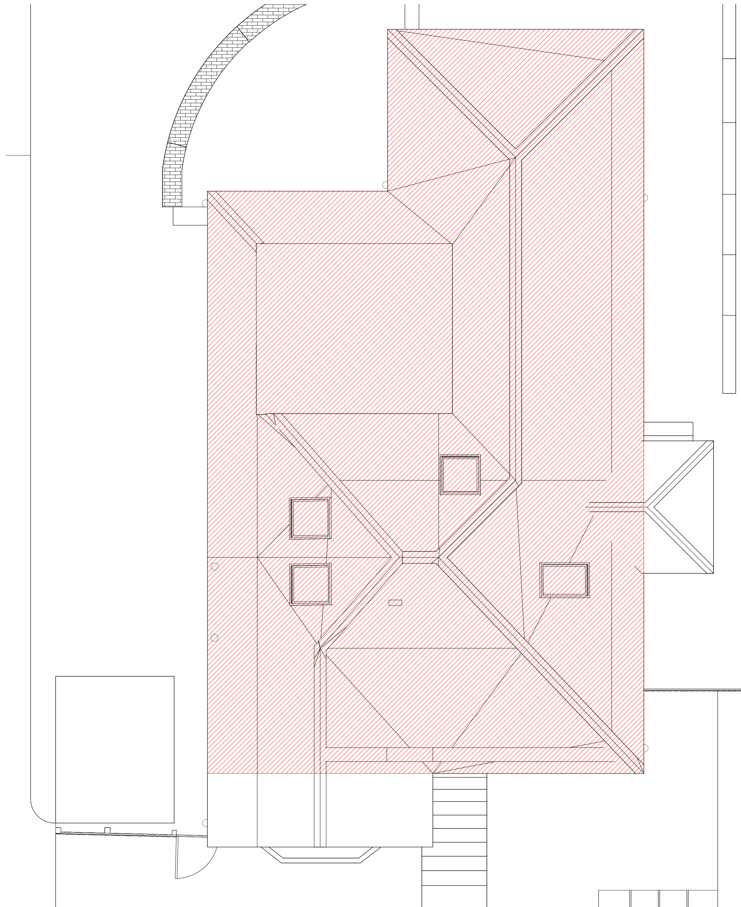
1 ROOF PLAN - AS EXISTING 1:50
