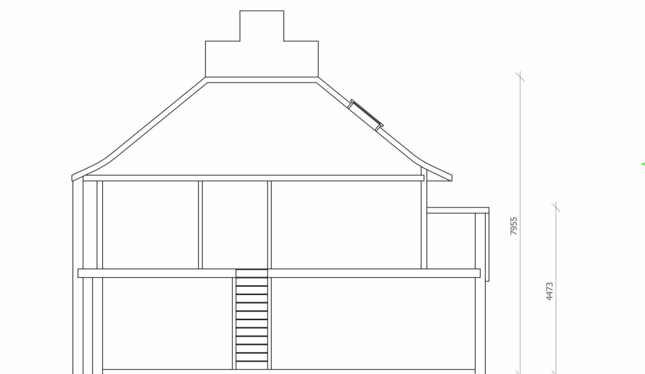
Existing Right Side Section
