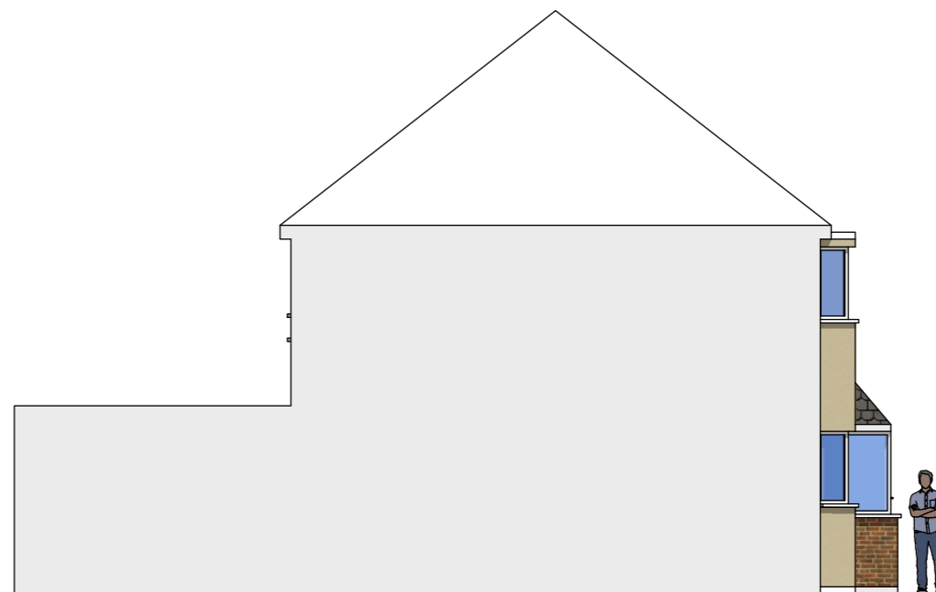
EXISTING LEFT ELEVATION SCALE 1:100 @ A3
