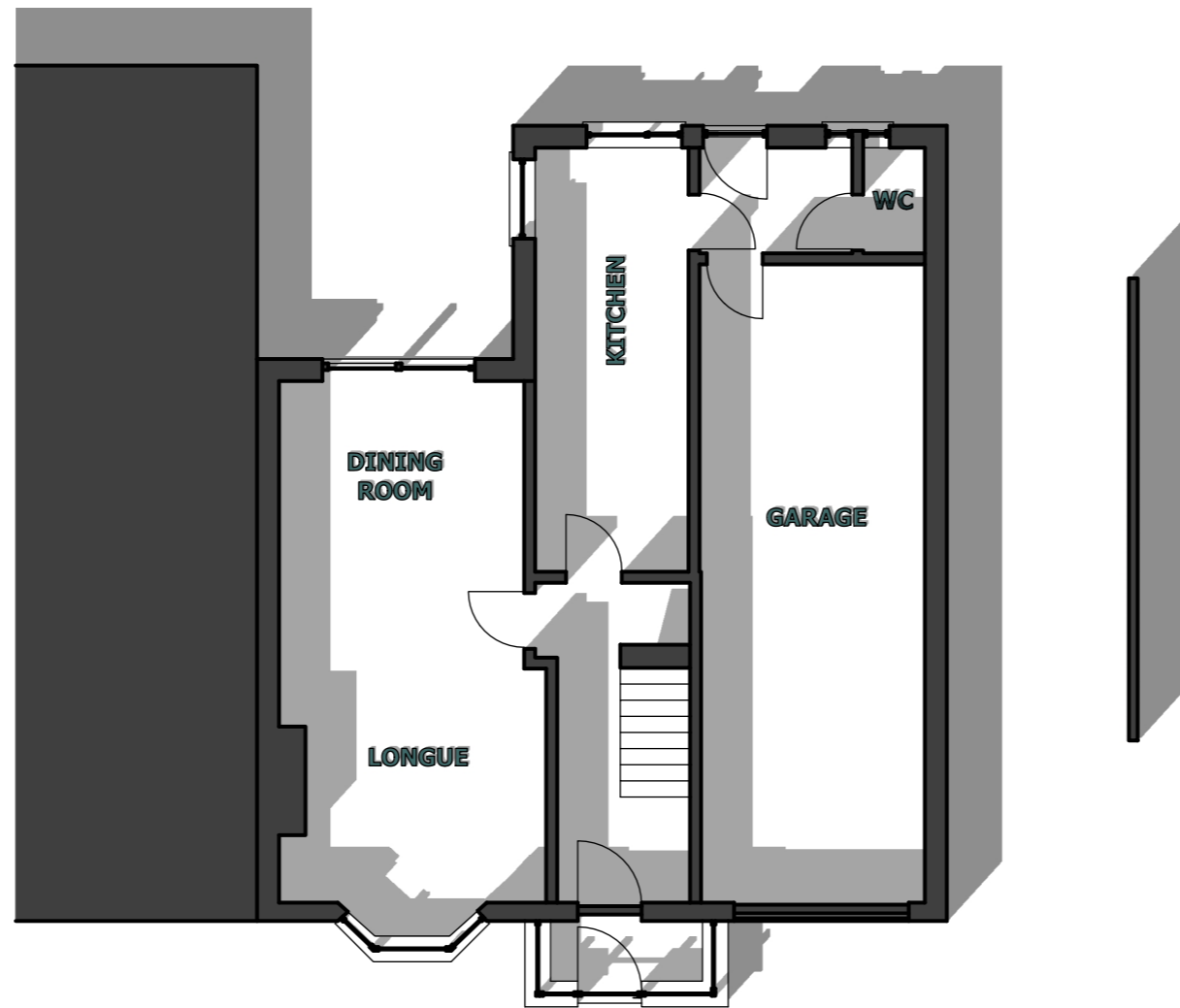
EXISTING GROUND FLOOR PLAN SCALE 1:100 @ A3
