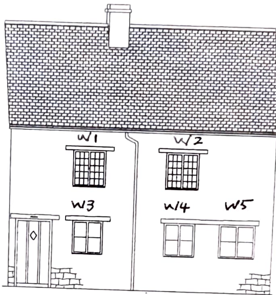
existing and proposed front elevation
