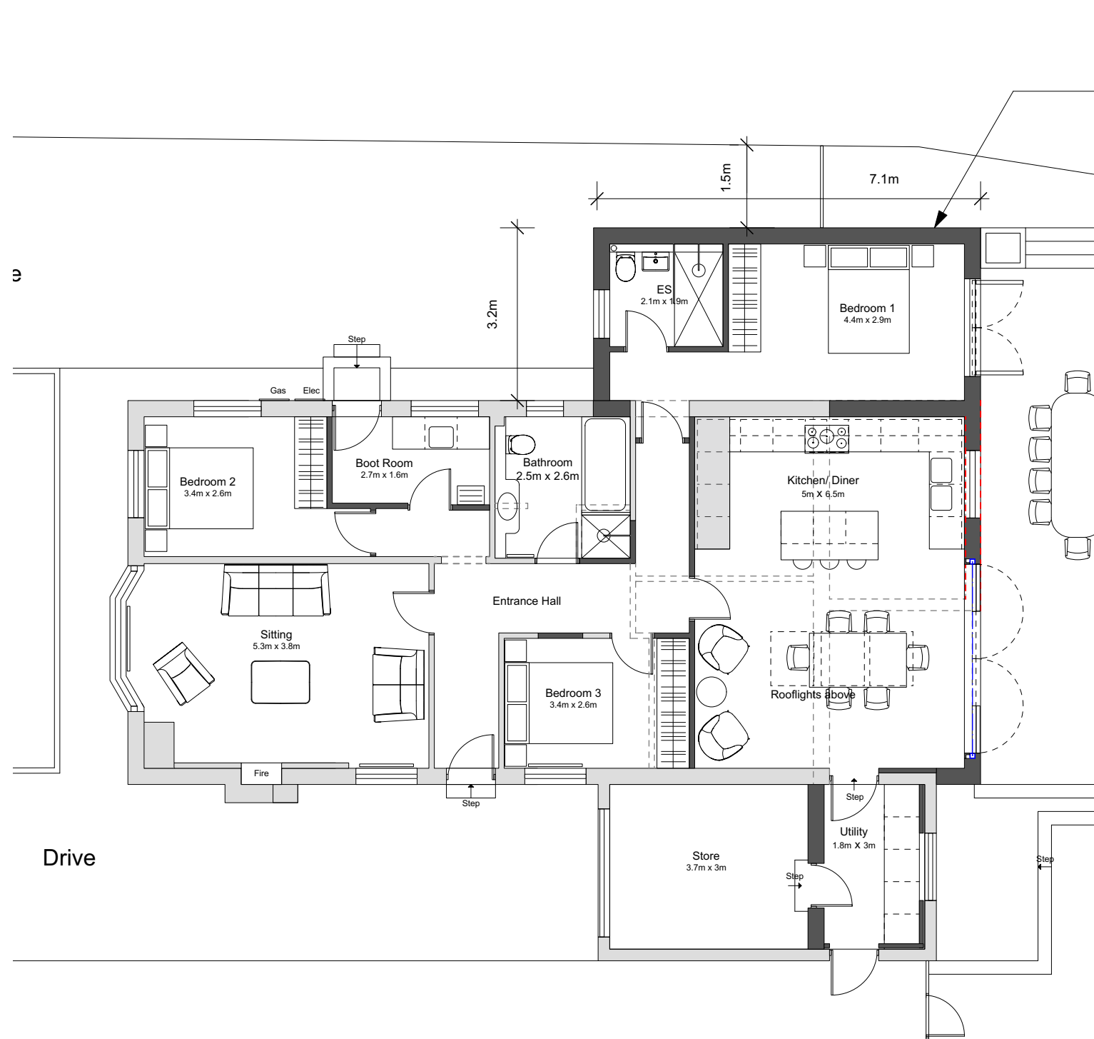
1 Ground Floor Plan Scale: 1:100
