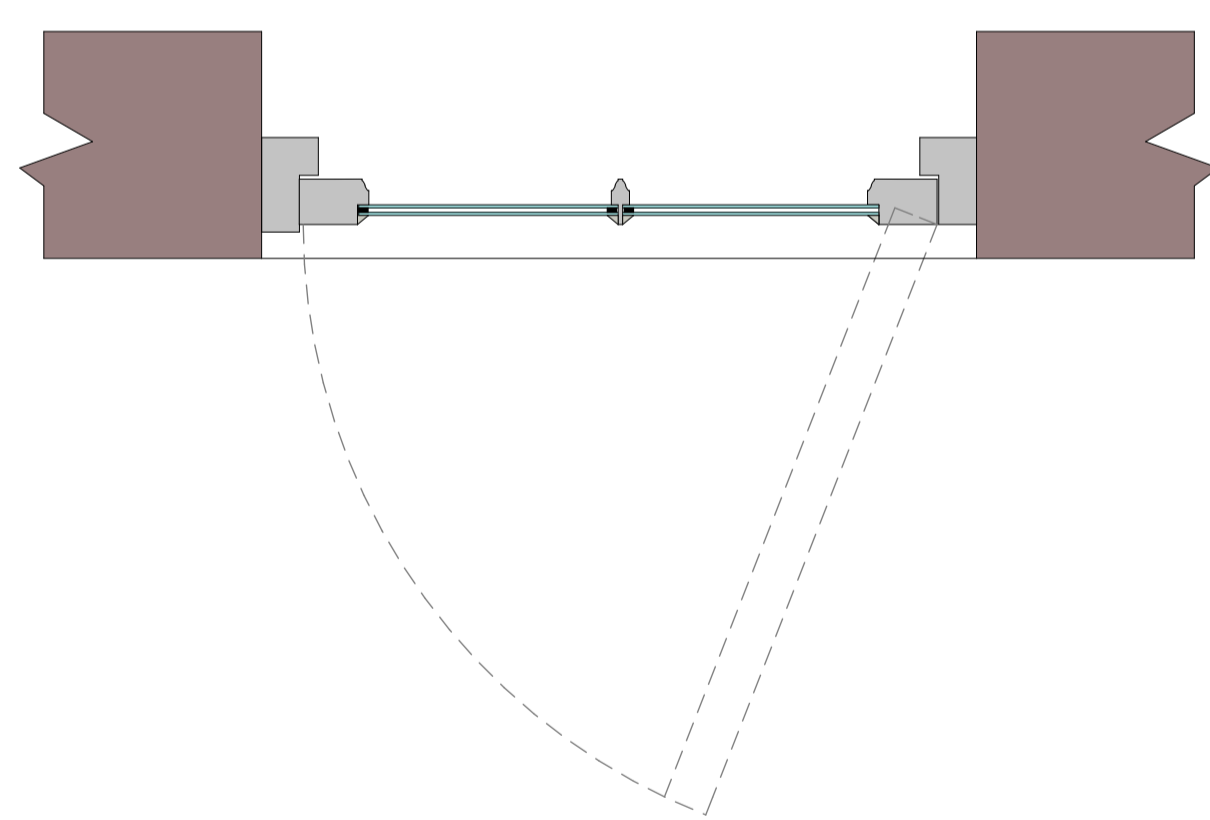
DOOR 'D1' PART GLAZED
