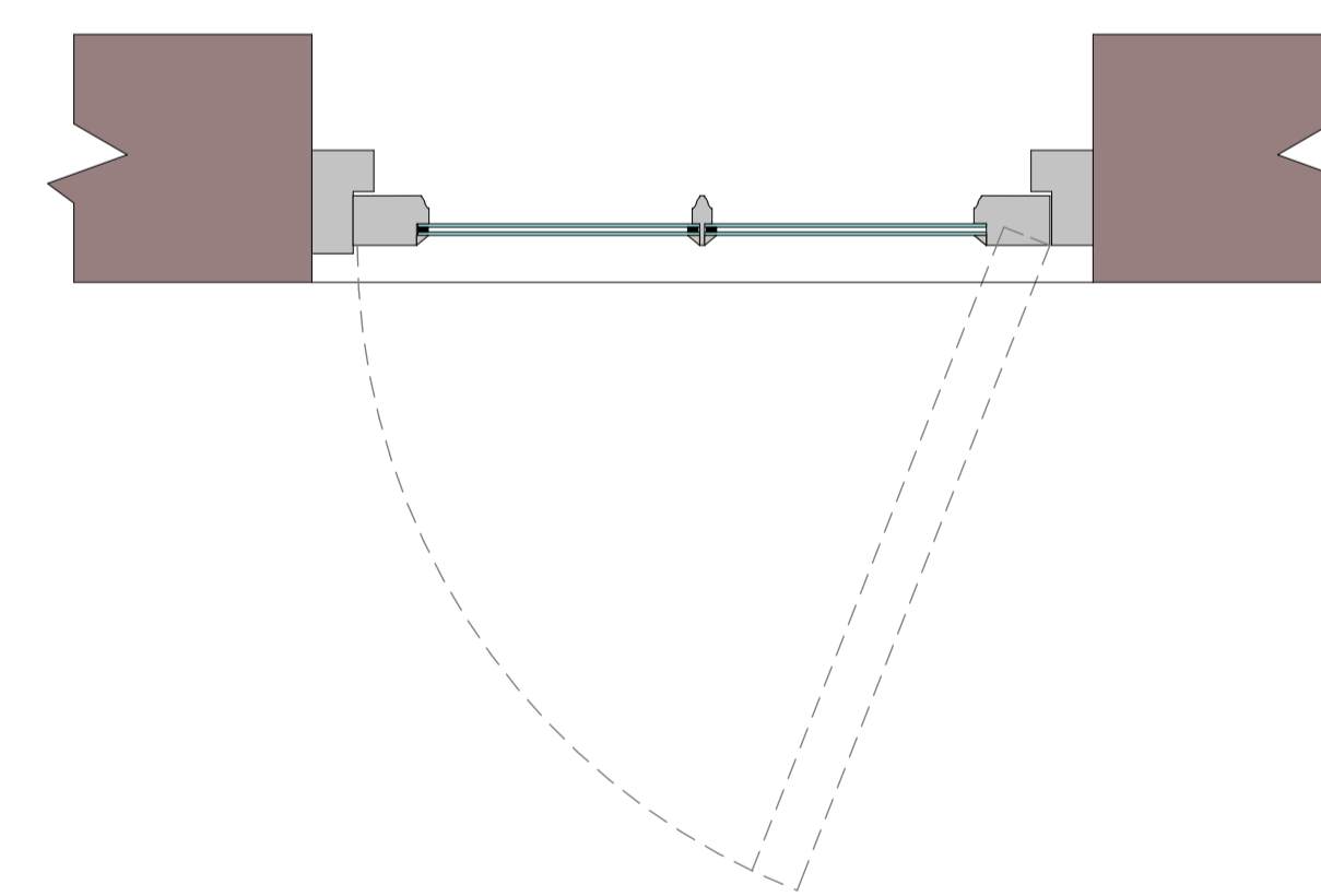
DOOR 'D2' PART GLAZED
