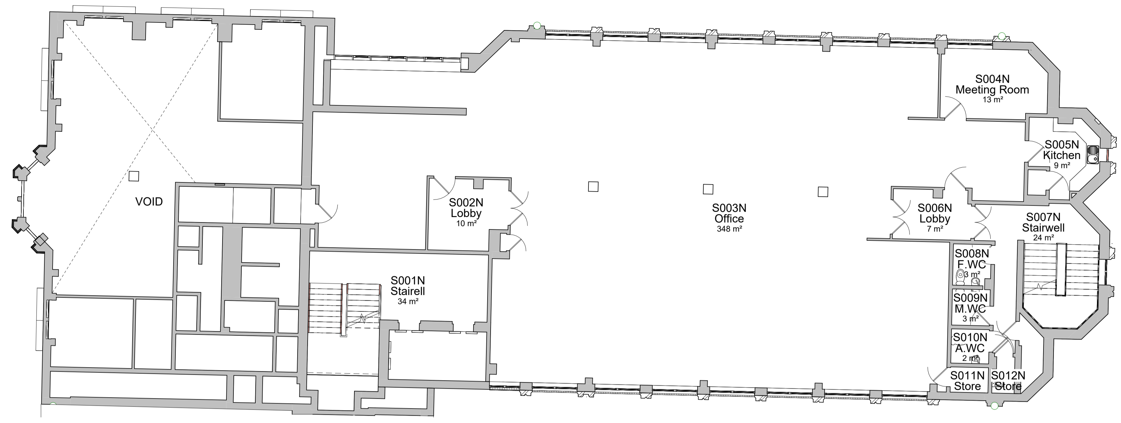
EX_02_Second Floor Plan_Intermediate Level (Extension)
