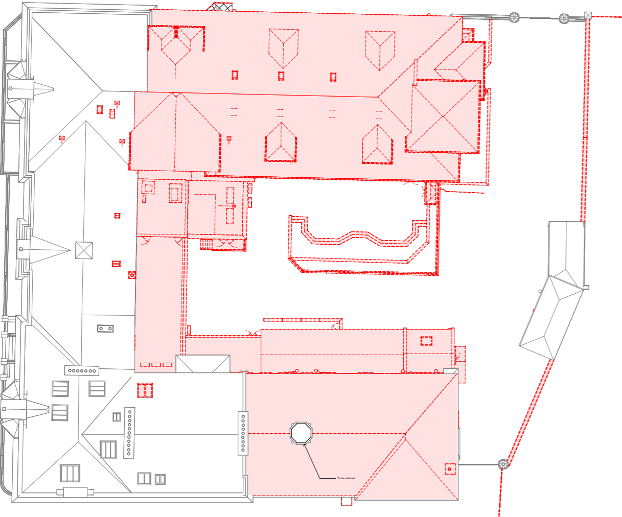
DM_05 Roof Plan
