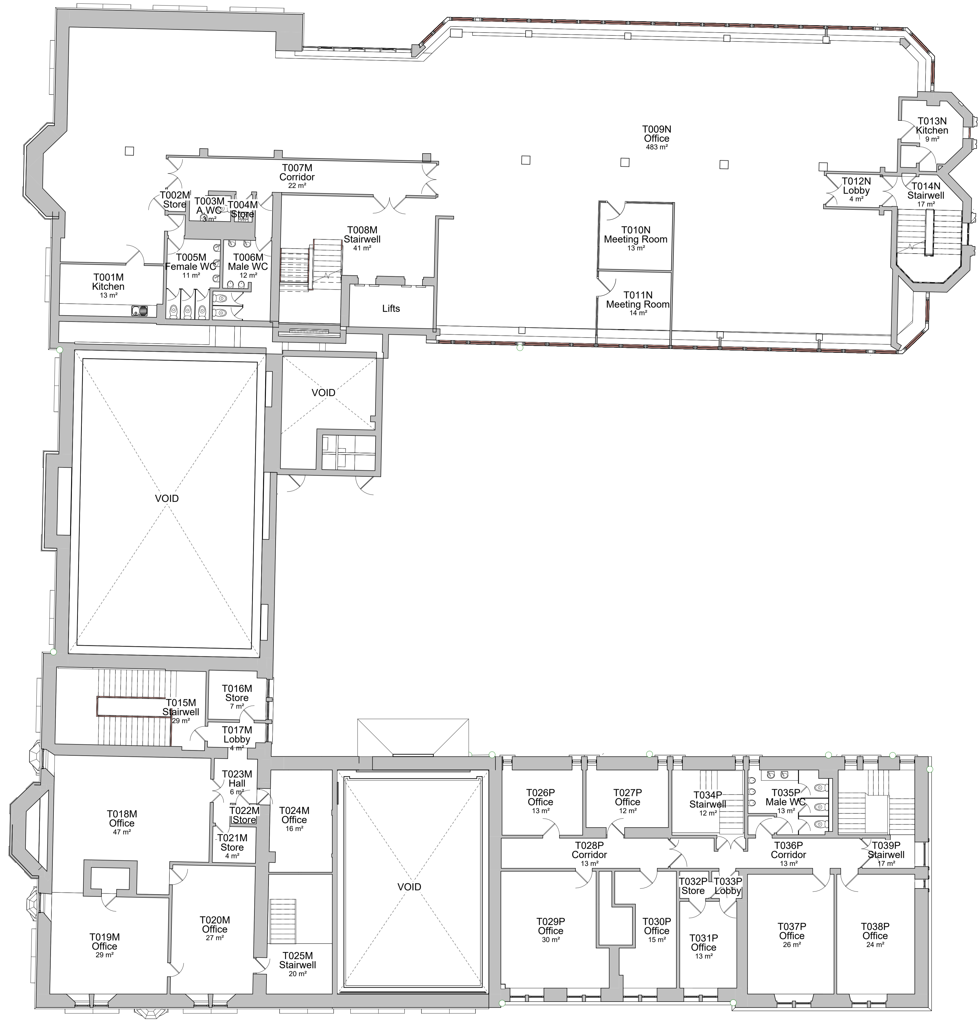
EX_03_Third Floor Plan (Extension) Second Floor Plan (Main Building)
