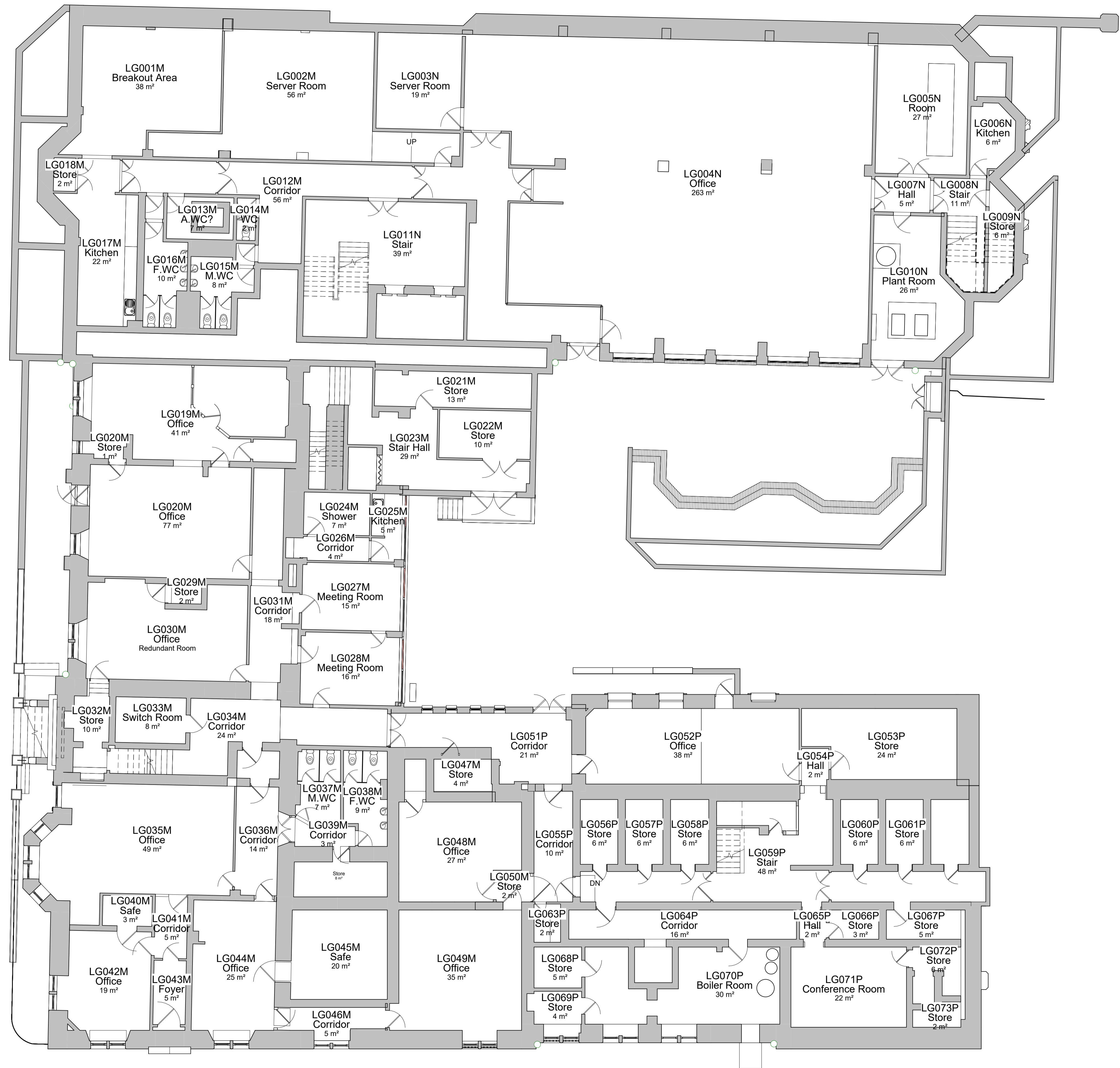
EX_-1_Lower Ground Floor Plan
