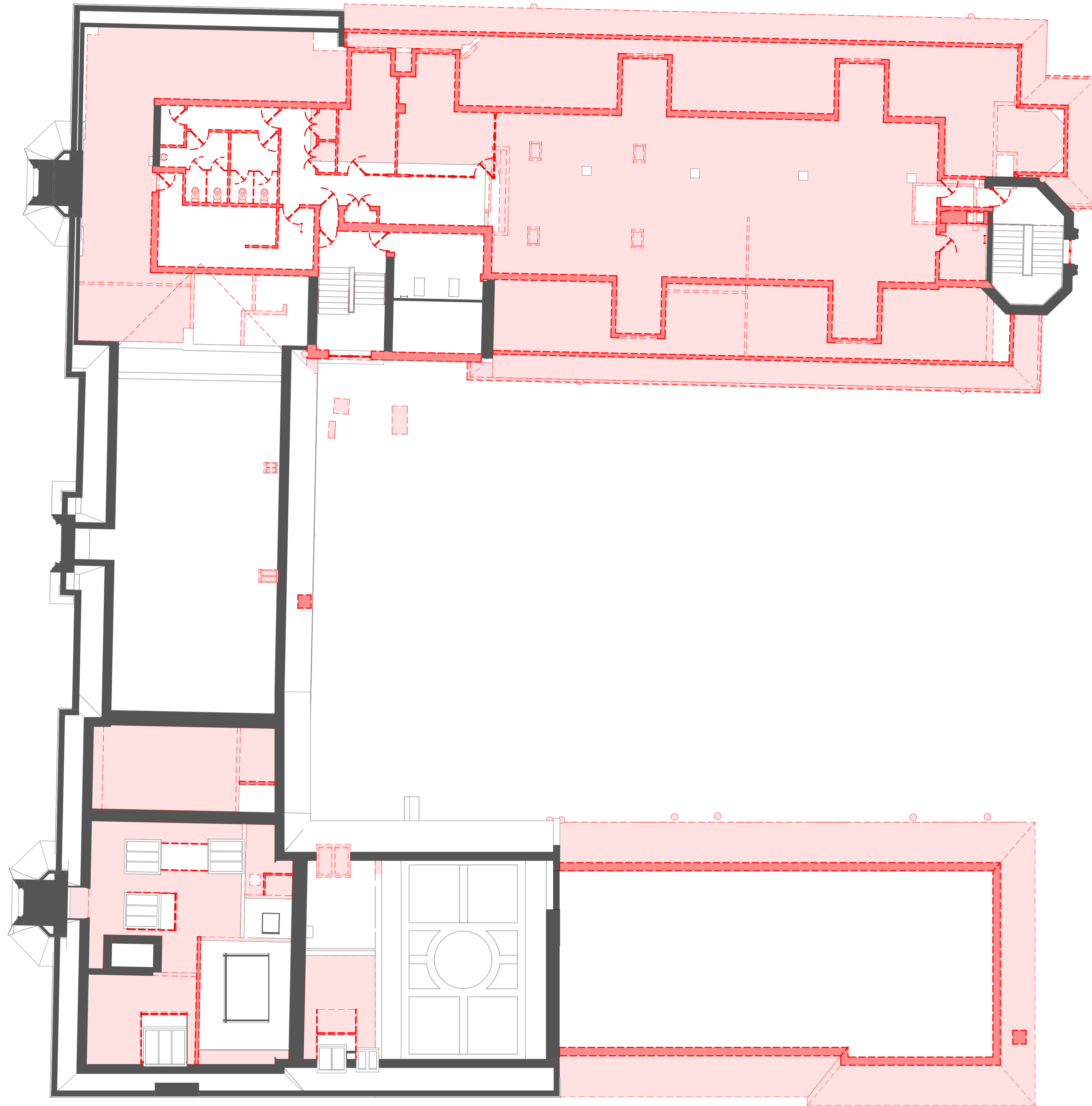
DM_04_Fourth Floor Plan (Extension) 1 : 100
