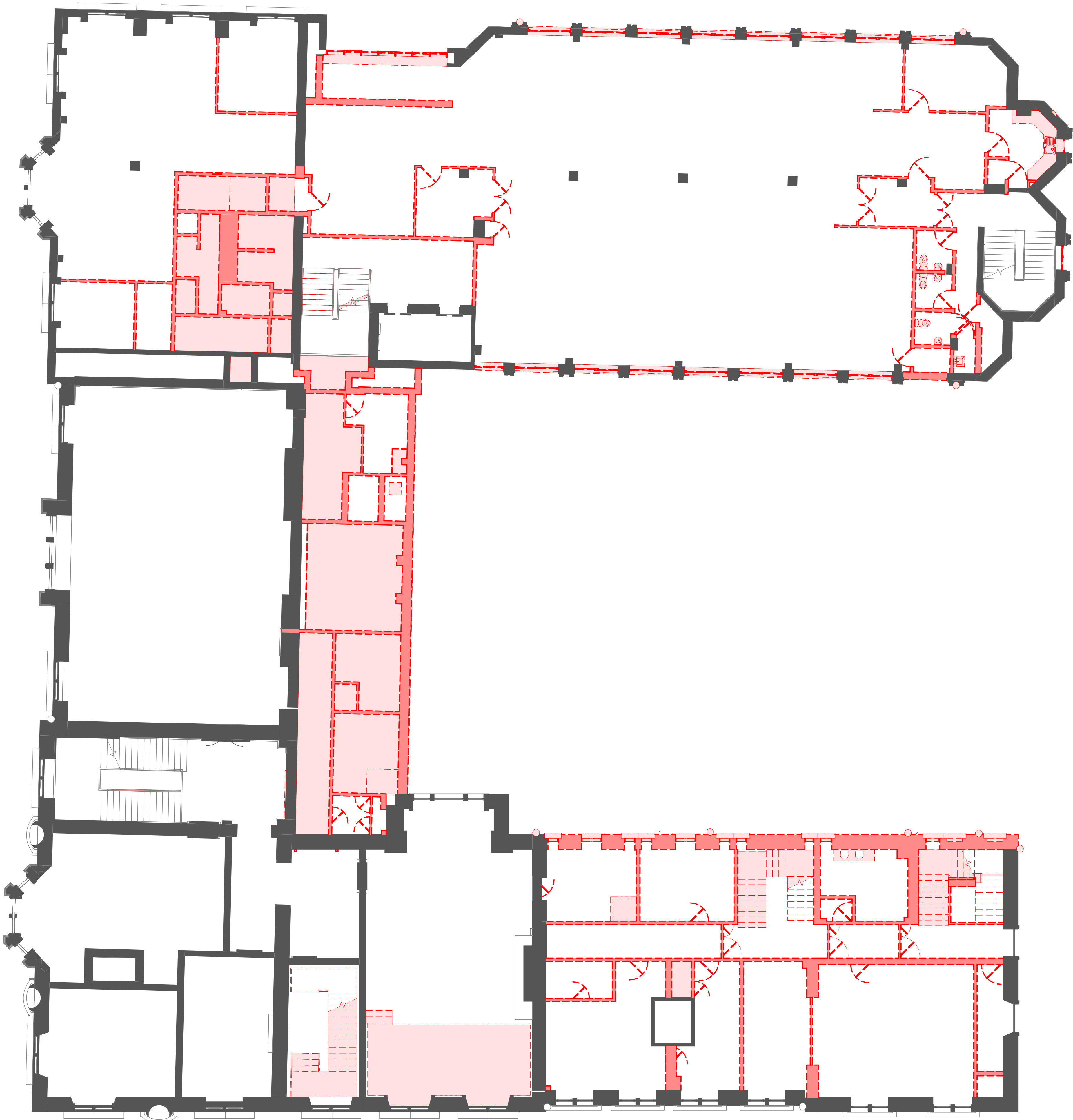
DM_02_Second Floor Plan_ Intermediate Level (Extension) 1 : 100
