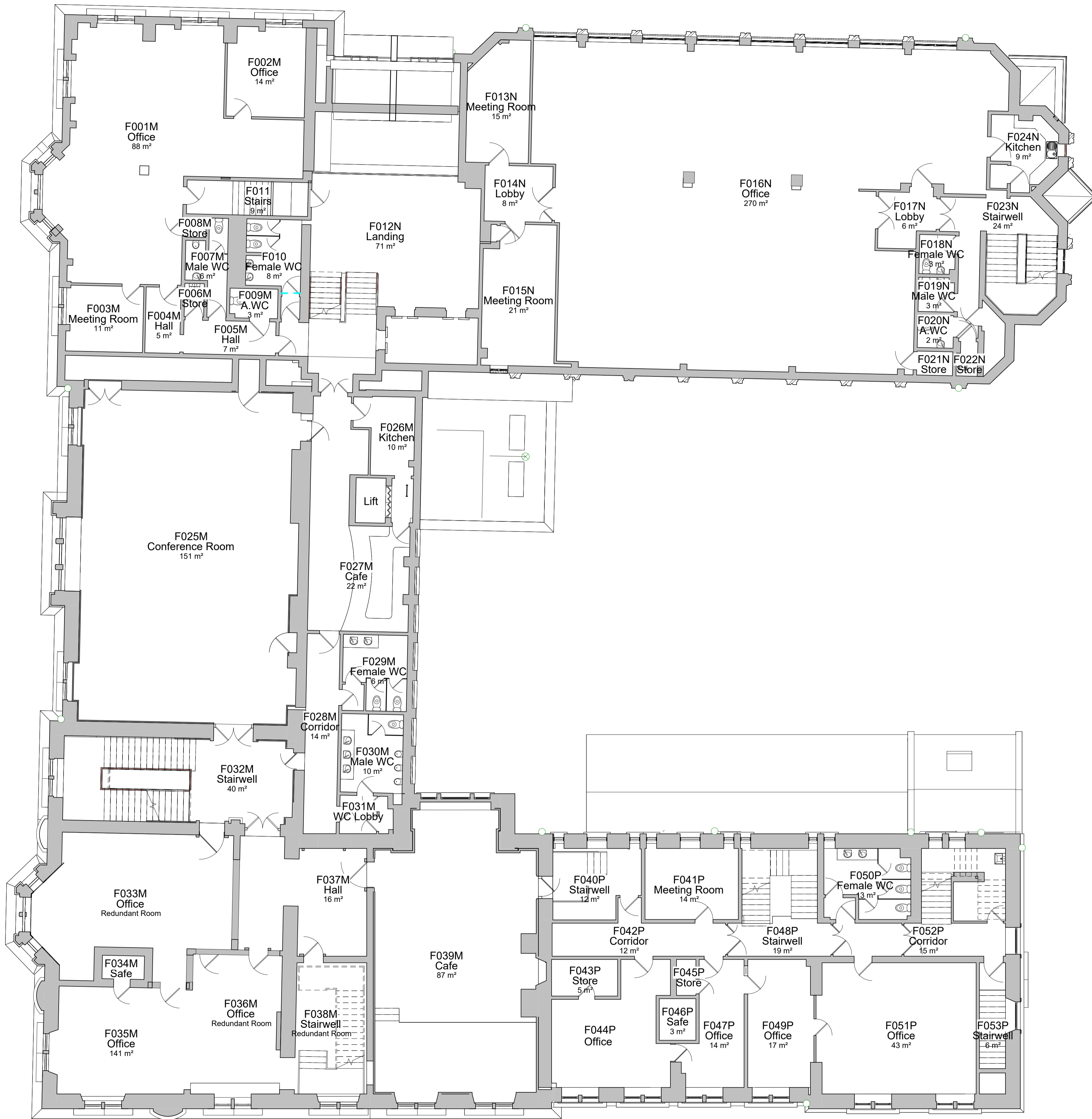
EX_01_First Floor Plan
