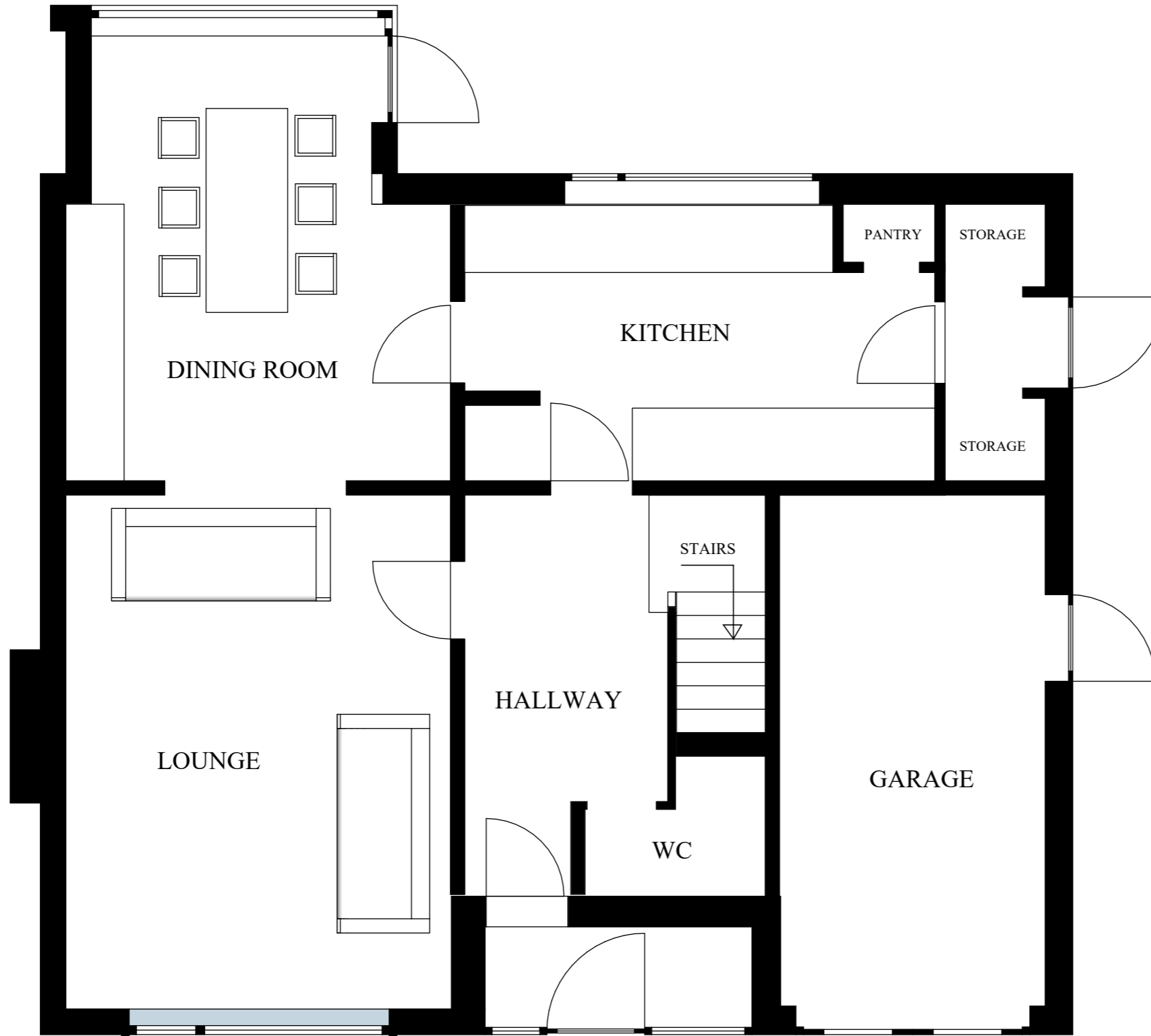
01 EXISTING GROUND FLOOR PLAN Scale: 1 : 50 @A3
