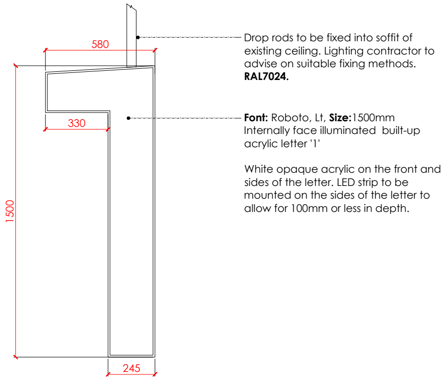
ILLUMINATED '1' SIGNAGE ELEVATION A @ 1:20
