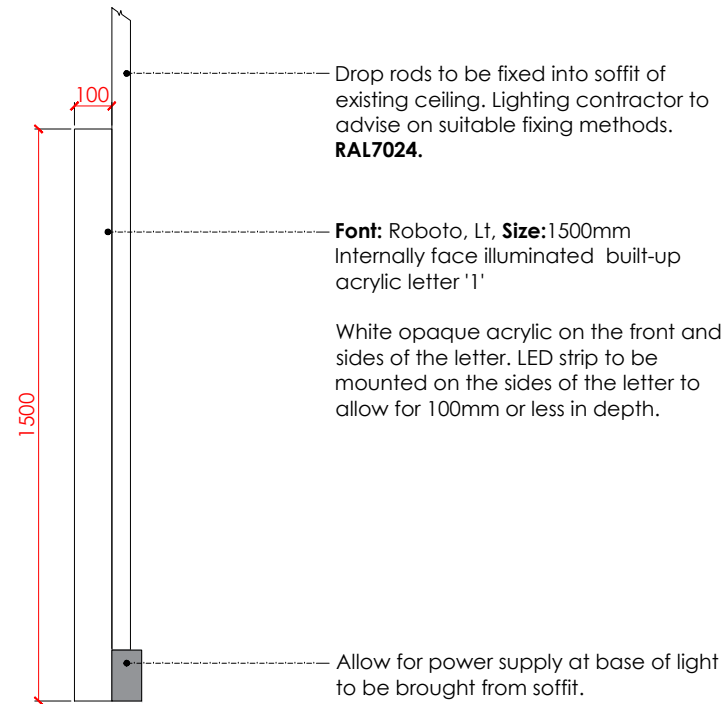
ILLUMINATED '1' SIGNAGE ELEVATION B @ 1:20
