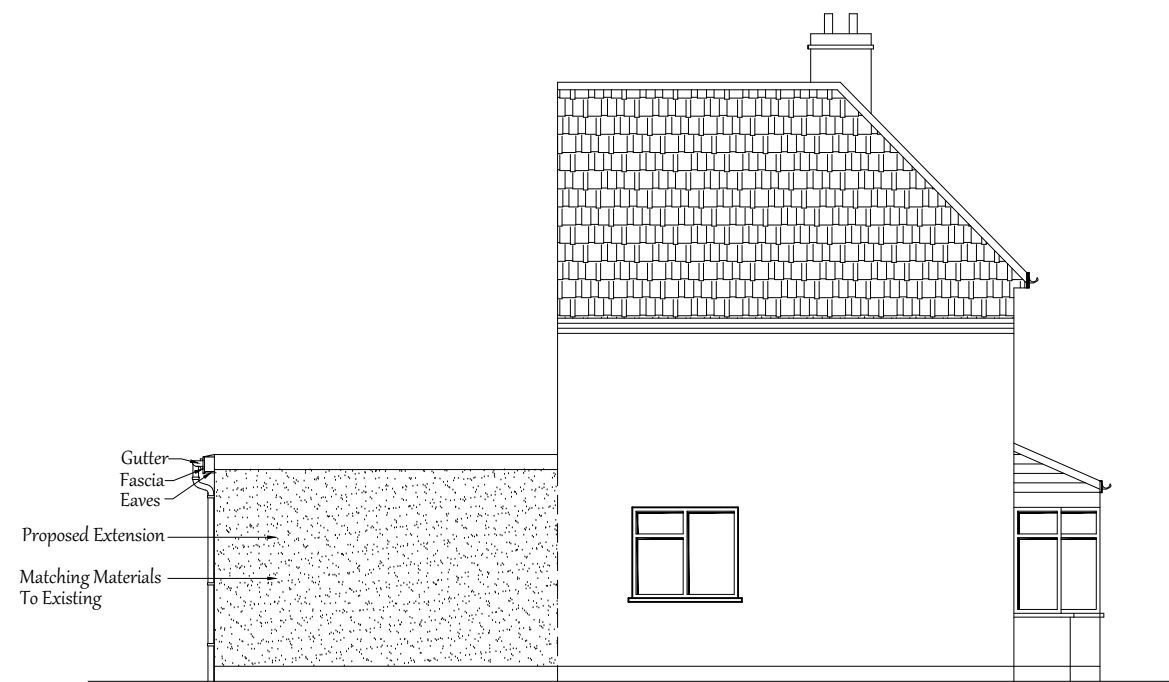
PROPOSED FLANK SIDE ELEVATION
