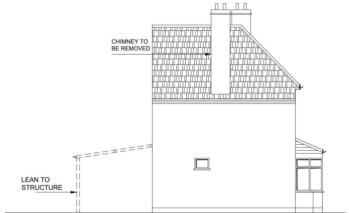
EXISTING FLANK SIDE ELEVATION
