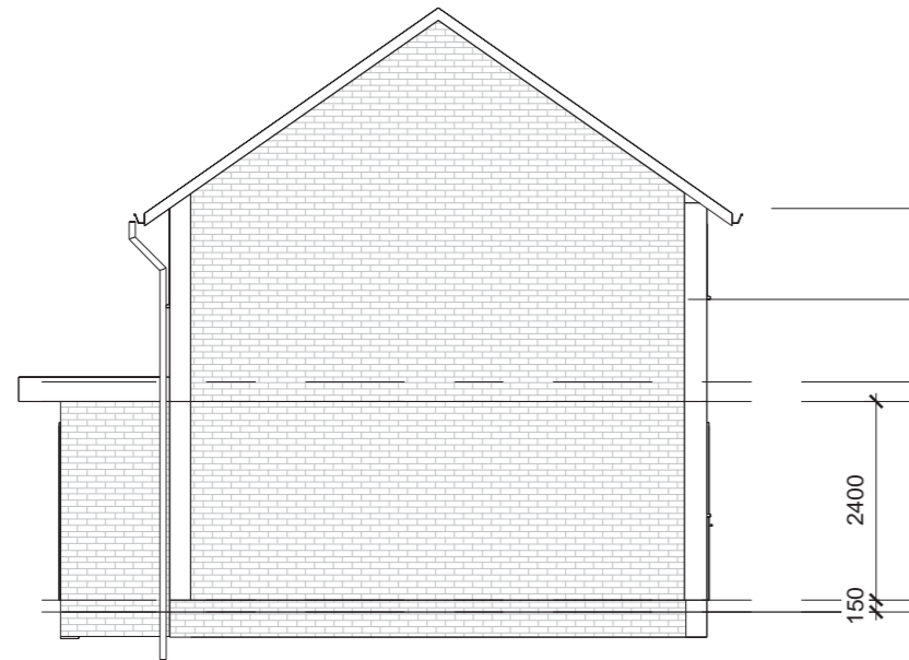
3 Existing Side Elevation 1 : 100
