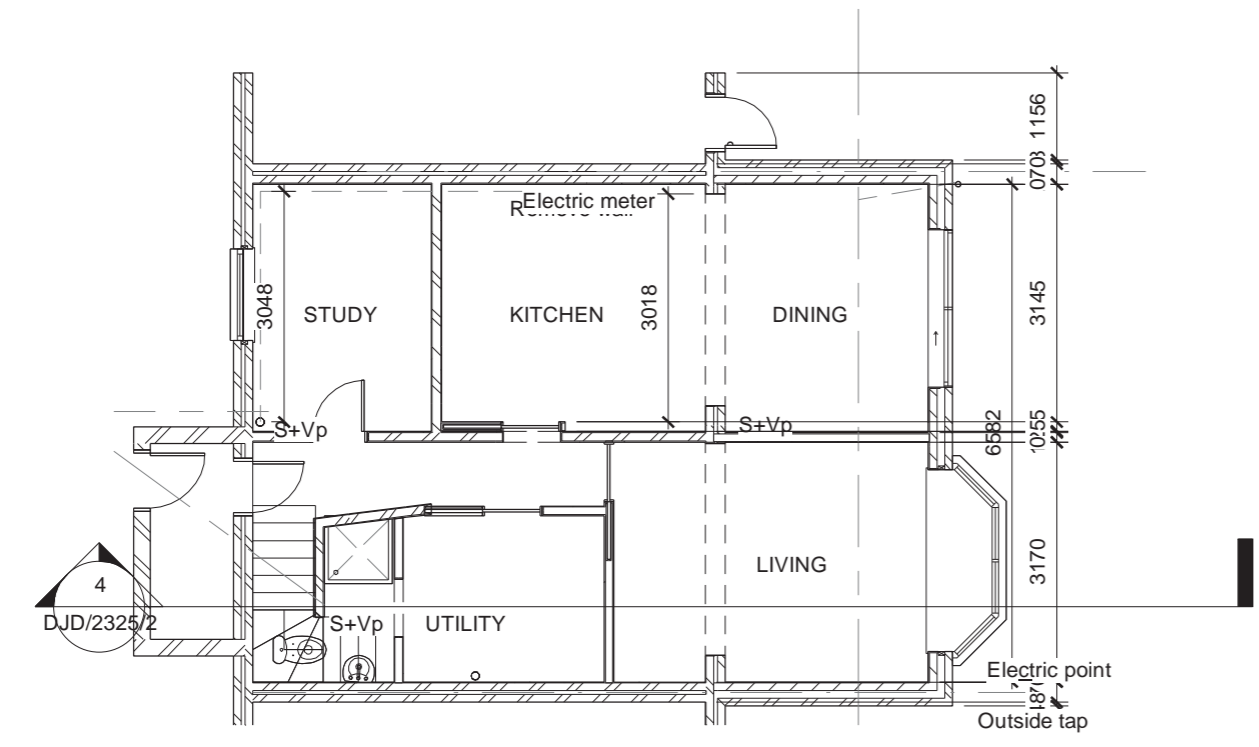
2 Ground Floor Proposed 1 : 100
