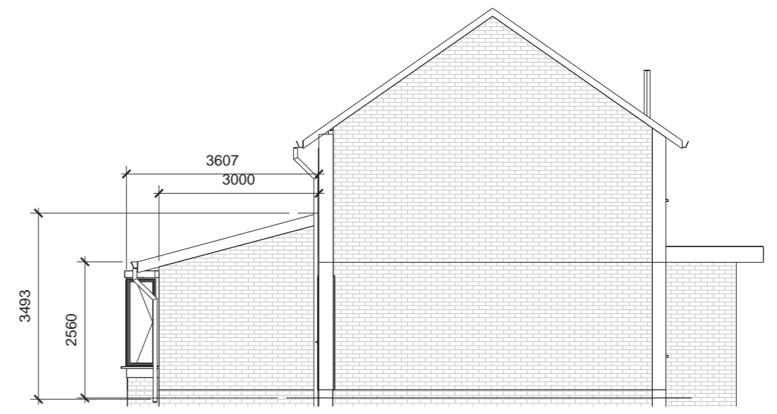
8 Proposed Adjoining Side Elevation 1 : 100
