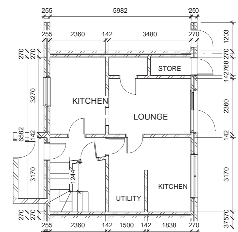
1 Ground Floor Existing 1 : 100
