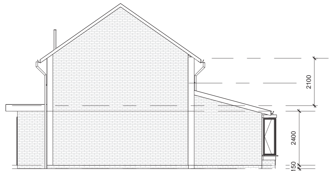
6 Proposed Side Elevation 1 : 100
