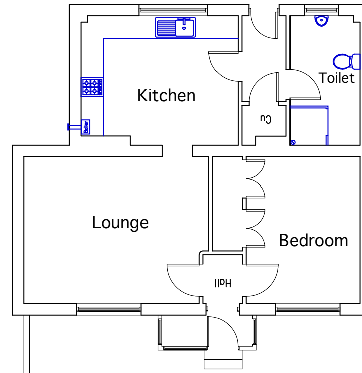
Ground Floor Plan as Existing
