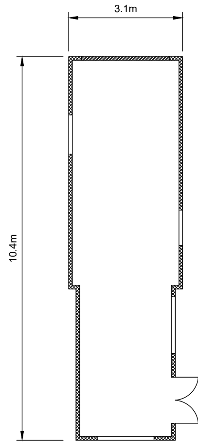
37 Newlands Copse - Garage Existing Floor Plan (Scale = 1:100)
