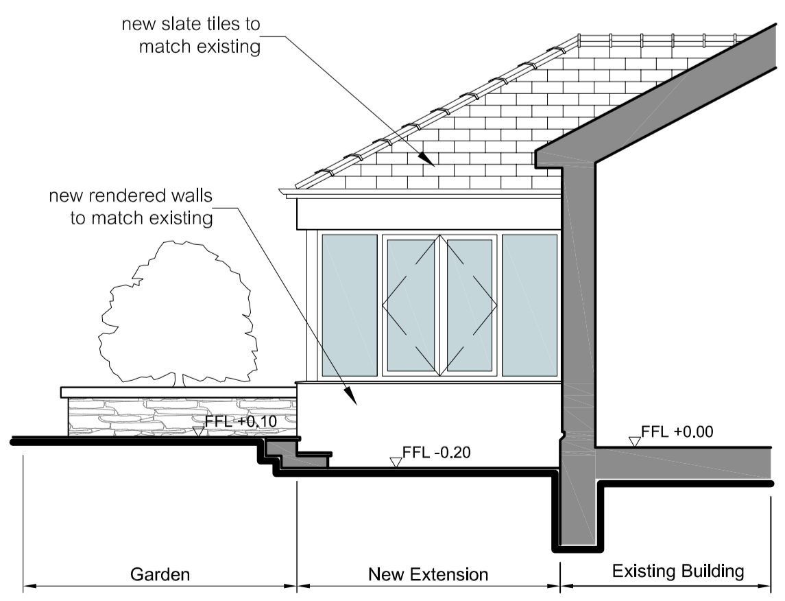
Proposed Southwest Elevation 1:50
