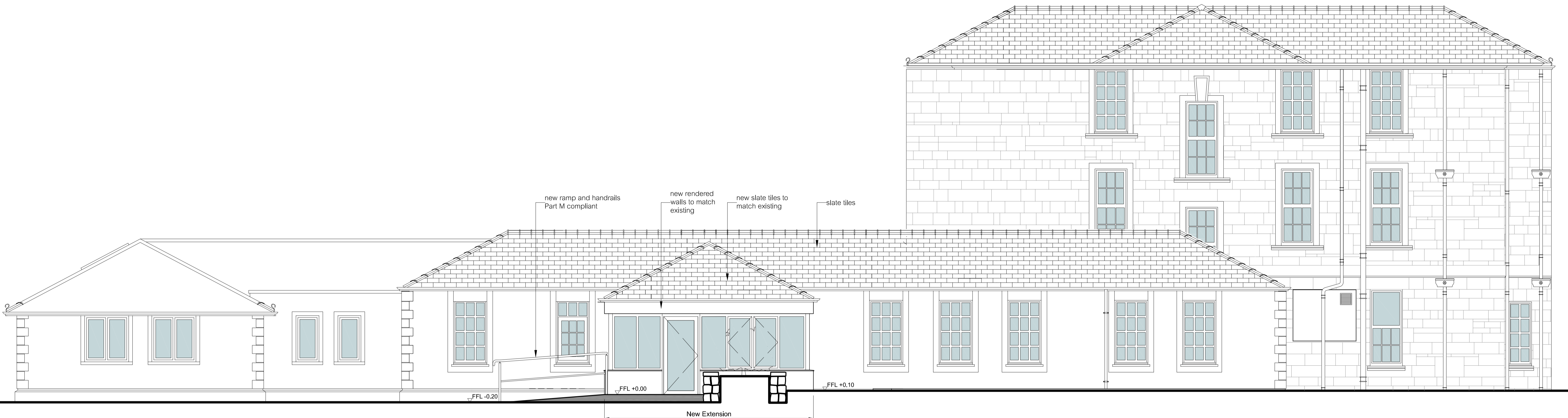
Proposed Northwest Elevation 1:50
