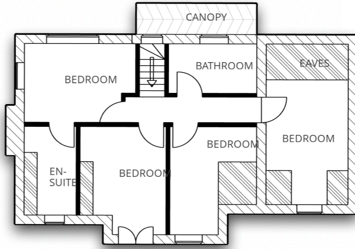
First Floor Scale - 1:50
