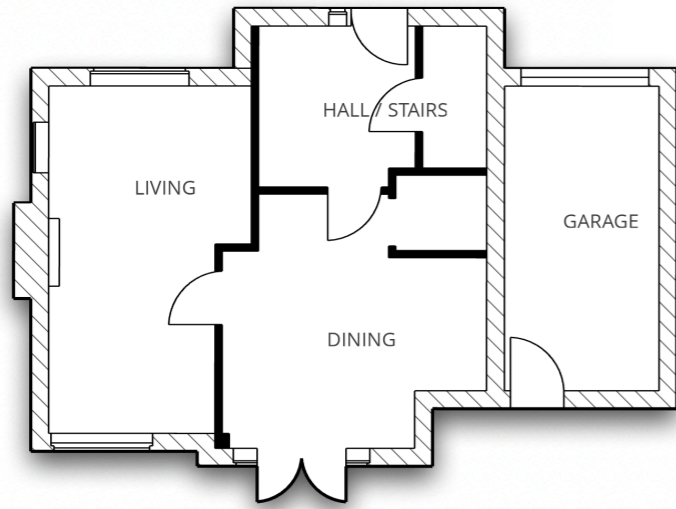
Ground Floor Scale - 1:50
